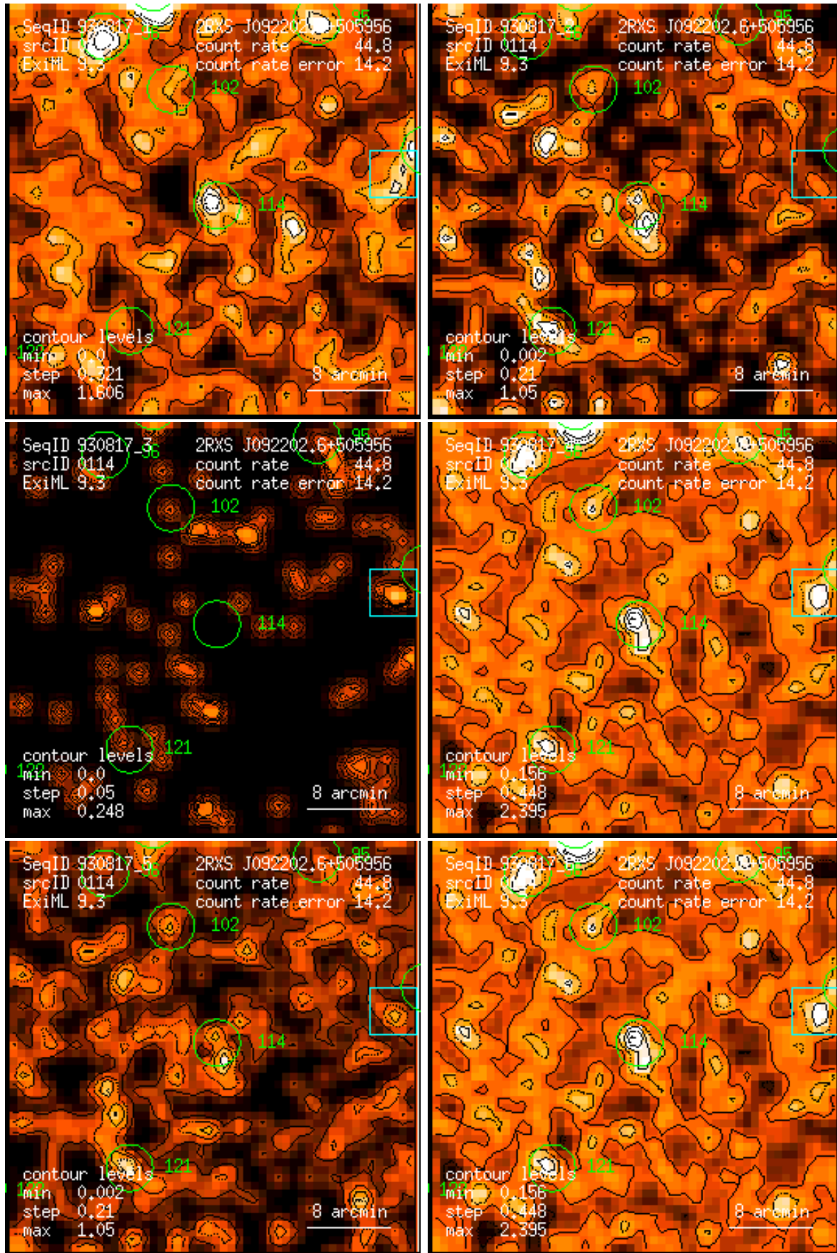
Figure 114: RASS 930817: detection 0114: band rate images, Gaussian filter: (1) PSPC channels 11 – 41, (2) 52 – 90, (3) 91 – 201, (4) 11 – 235, (5) 52 – 201, (6) 11 – 201. Broad band rates in counts/ks. Band rate contour levels in counts/ks/arcmin 2 .
