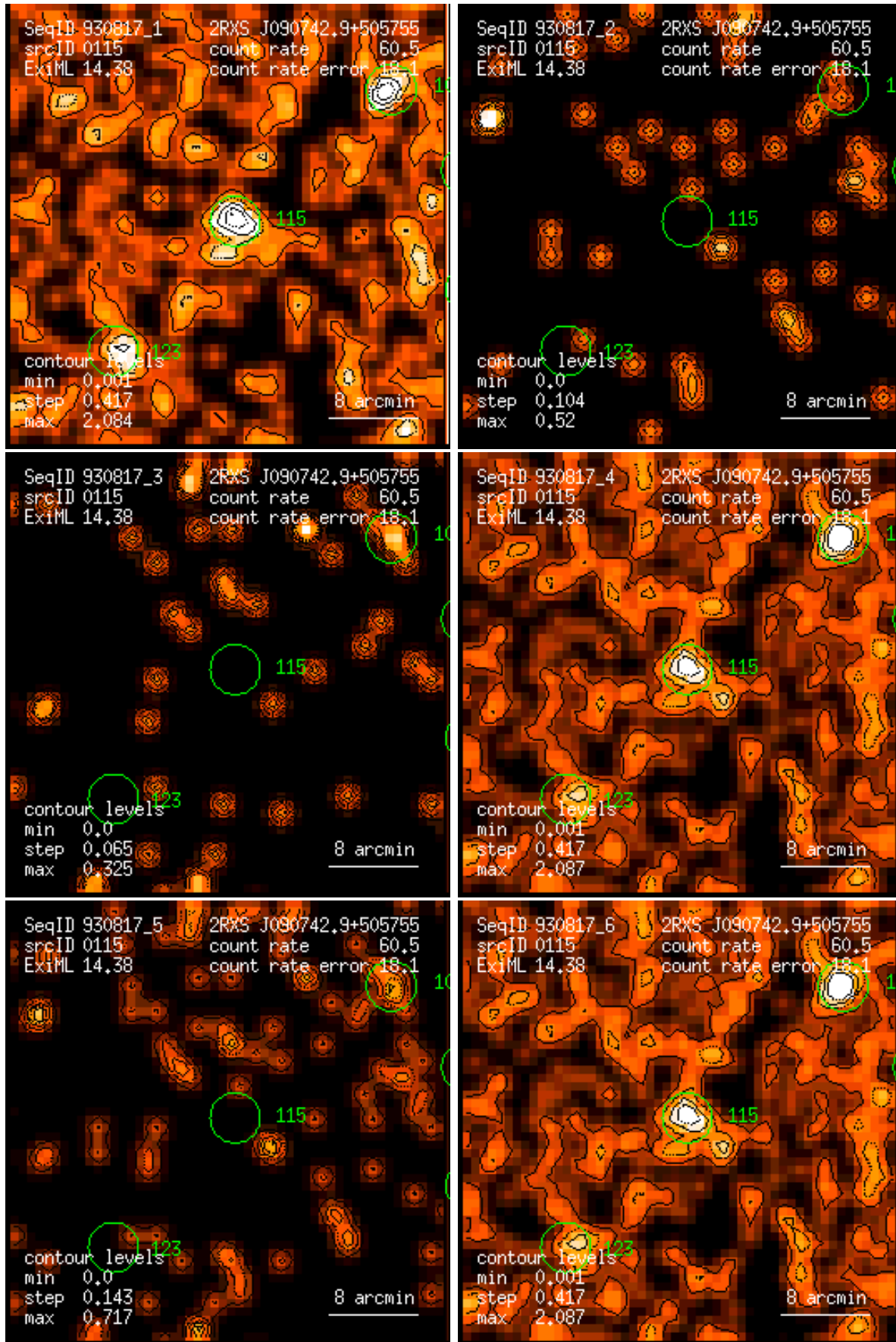
Figure 115: RASS 930817: detection 0115: band rate images, Gaussian filter: (1) PSPC channels 11 – 41, (2) 52 – 90, (3) 91 – 201, (4) 11 – 235, (5) 52 – 201, (6) 11 – 201. Broad band rates in counts/ks. Band rate contour levels in counts/ks/arcmin 2 .
