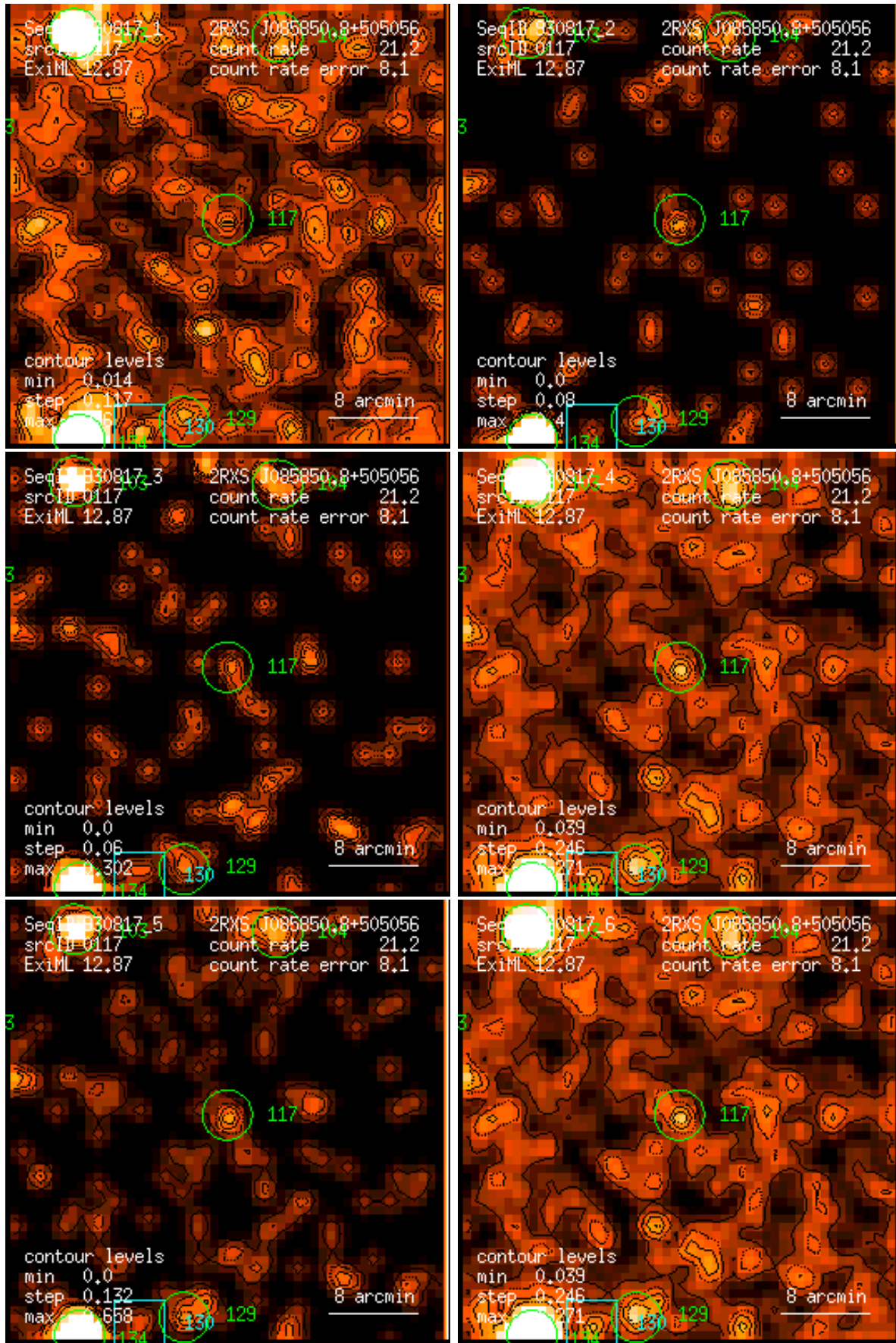
Figure 117: RASS 930817: detection 0117: band rate images, Gaussian filter: (1) PSPC channels 11 – 41, (2) 52 – 90, (3) 91 – 201, (4) 11 – 235, (5) 52 – 201, (6) 11 – 201. Broad band rates in counts/ks. Band rate contour levels in counts/ks/arcmin 2 .
