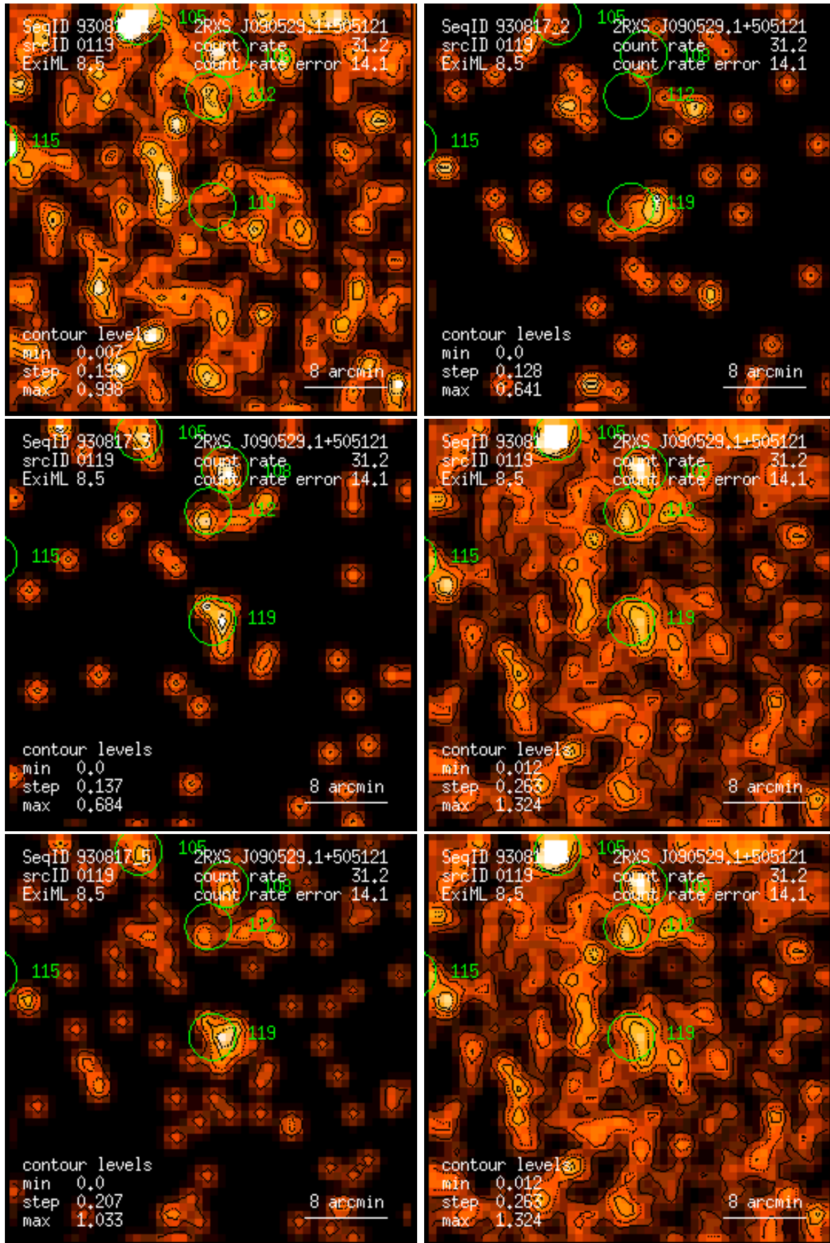
Figure 119: RASS 930817: detection 0119: band rate images, Gaussian filter: (1) PSPC channels 11 – 41, (2) 52 – 90, (3) 91 – 201, (4) 11 – 235, (5) 52 – 201, (6) 11 – 201. Broad band rates in counts/ks. Band rate contour levels in counts/ks/arcmin 2 .
