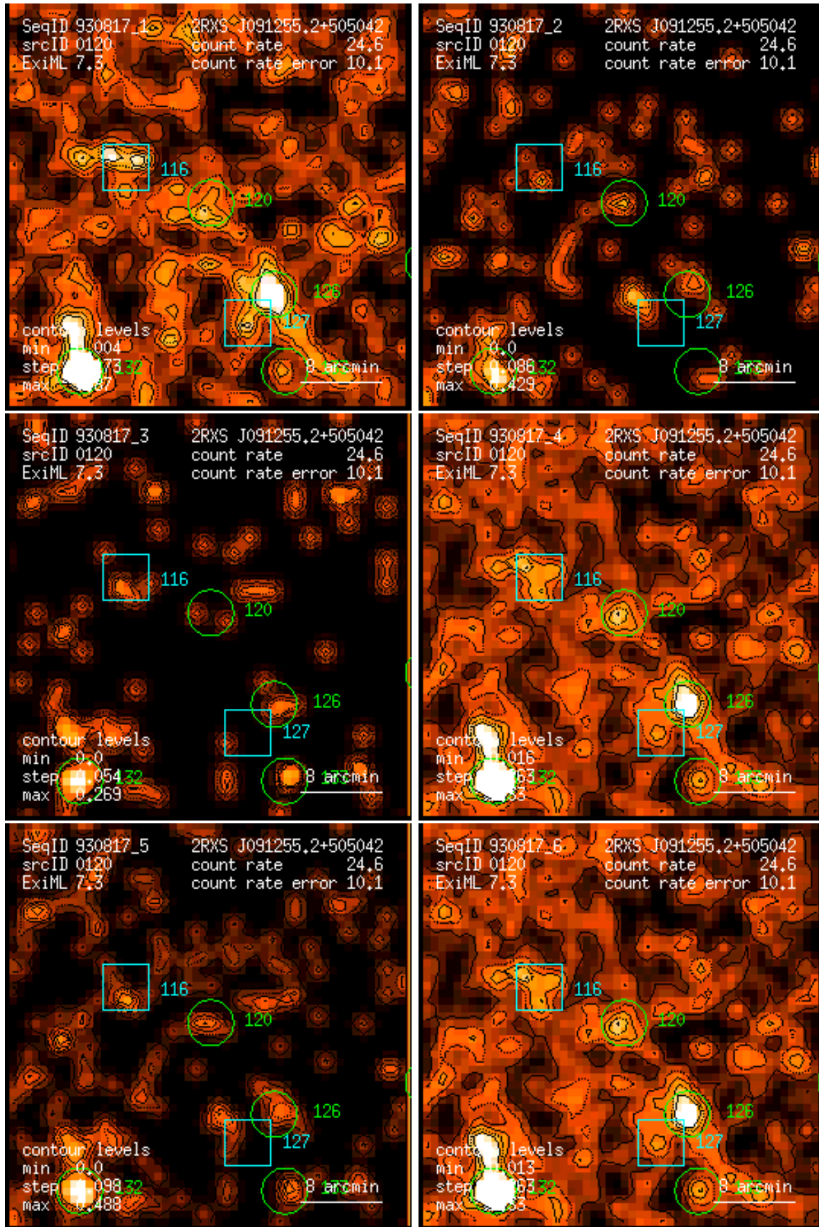
Figure 120: RASS 930817: detection 0120: band rate images, Gaussian filter: (1) PSPC channels 11 – 41, (2) 52 – 90, (3) 91 – 201, (4) 11 – 235, (5) 52 – 201, (6) 11 – 201. Broad band rates in counts/ks. Band rate contour levels in counts/ks/arcmin 2 .
