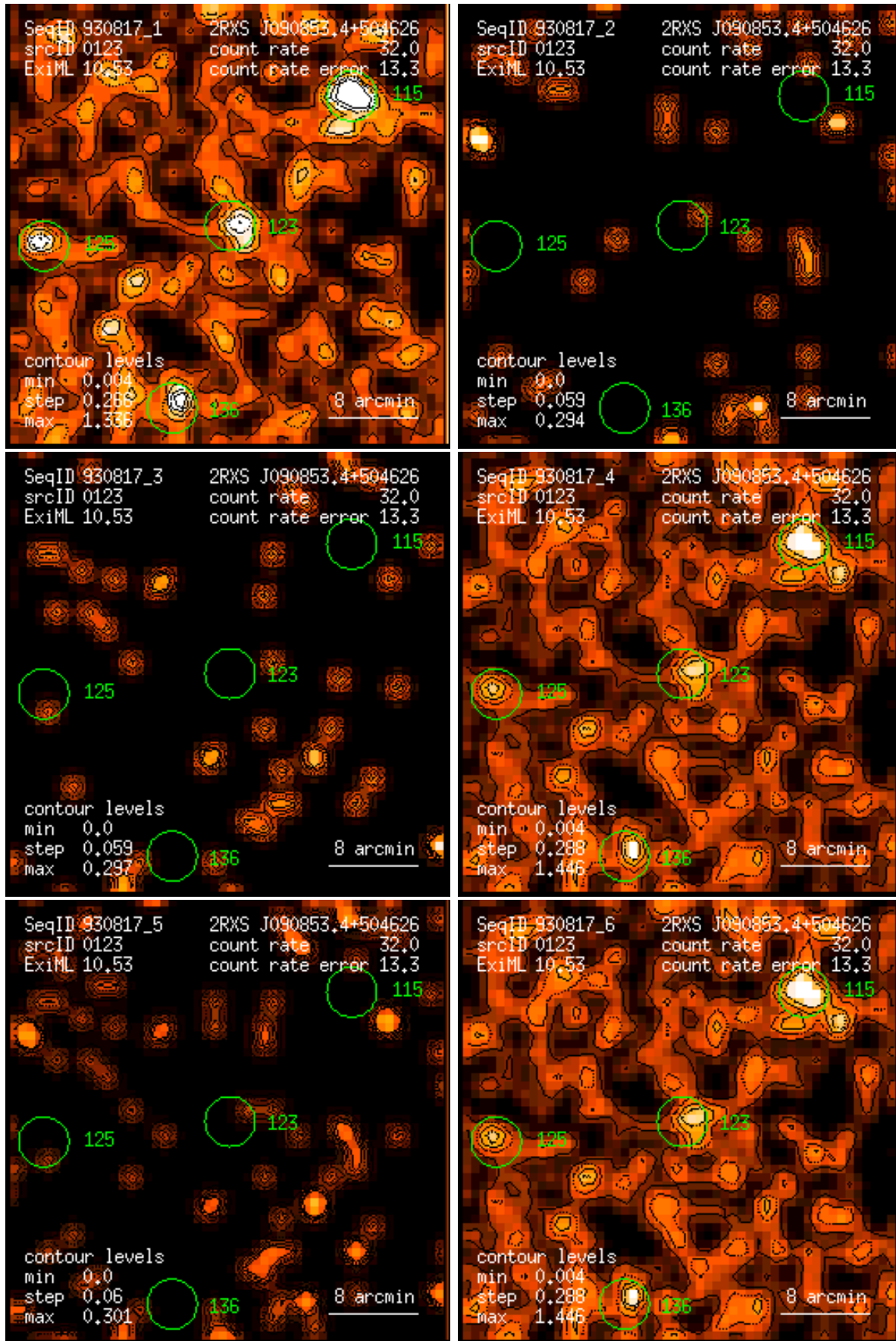
Figure 123: RASS 930817: detection 0123: band rate images, Gaussian filter: (1) PSPC channels 11 – 41, (2) 52 – 90, (3) 91 – 201, (4) 11 – 235, (5) 52 – 201, (6) 11 – 201. Broad band rates in counts/ks. Band rate contour levels in counts/ks/arcmin 2 .
