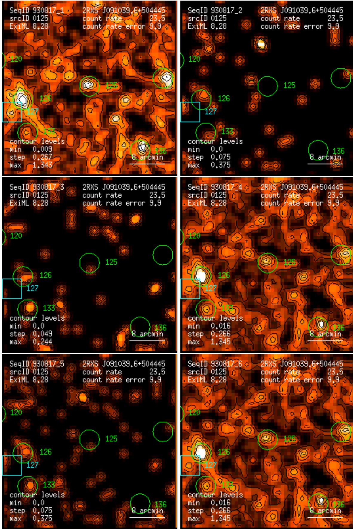
Figure 125: RASS 930817: detection 0125: band rate images, Gaussian filter: (1) PSPC channels 11 – 41, (2) 52 – 90, (3) 91 – 201, (4) 11 – 235, (5) 52 – 201, (6) 11 – 201. Broad band rates in counts/ks. Band rate contour levels in counts/ks/arcmin 2 .
