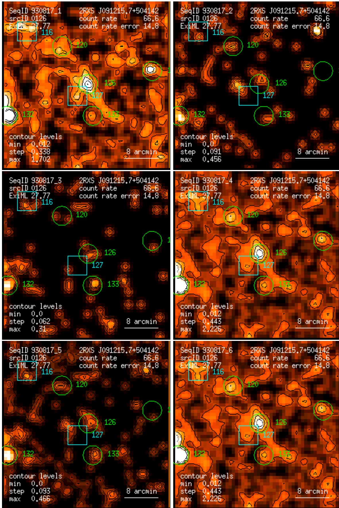
Figure 126: RASS 930817: detection 0126: band rate images, Gaussian filter: (1) PSPC channels 11 – 41, (2) 52 – 90, (3) 91 – 201, (4) 11 – 235, (5) 52 – 201, (6) 11 – 201. Broad band rates in counts/ks. Band rate contour levels in counts/ks/arcmin 2 .
