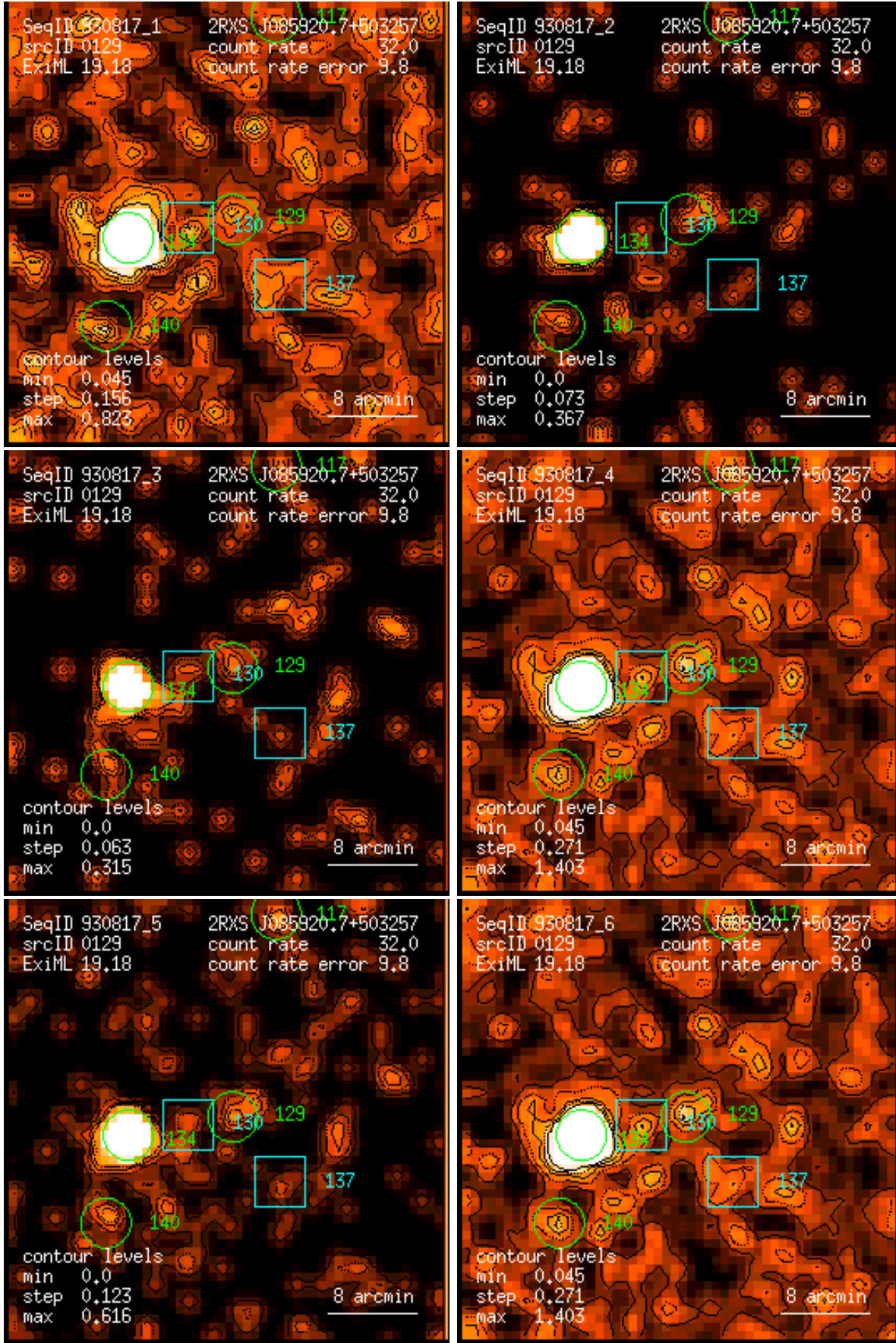
Figure 129: RASS 930817: detection 0129: band rate images, Gaussian filter: (1) PSPC channels 11 – 41, (2) 52 – 90, (3) 91 – 201, (4) 11 – 235, (5) 52 – 201, (6) 11 – 201. Broad band rates in counts/ks. Band rate contour levels in counts/ks/arcmin 2 .
