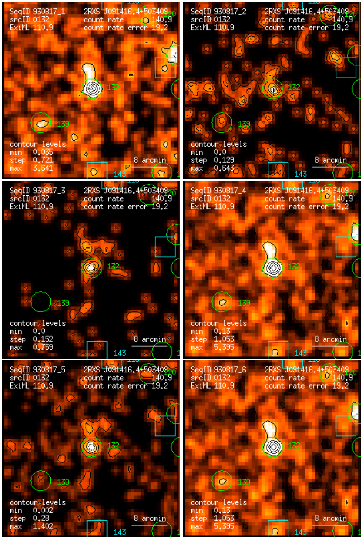
Figure 132: RASS 930817: detection 0132: band rate images, Gaussian filter: (1) PSPC channels 11 – 41, (2) 52 – 90, (3) 91 – 201, (4) 11 – 235, (5) 52 – 201, (6) 11 – 201. Broad band rates in counts/ks. Band rate contour levels in counts/ks/arcmin 2 .
