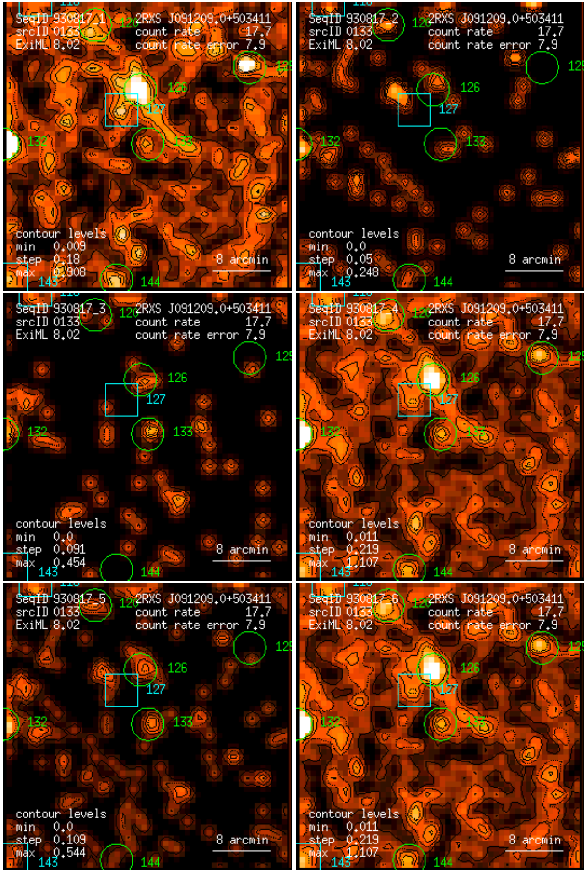
Figure 133: RASS 930817: detection 0133: band rate images, Gaussian filter: (1) PSPC channels 11 – 41, (2) 52 – 90, (3) 91 – 201, (4) 11 – 235, (5) 52 – 201, (6) 11 – 201. Broad band rates in counts/ks. Band rate contour levels in counts/ks/arcmin 2 .
