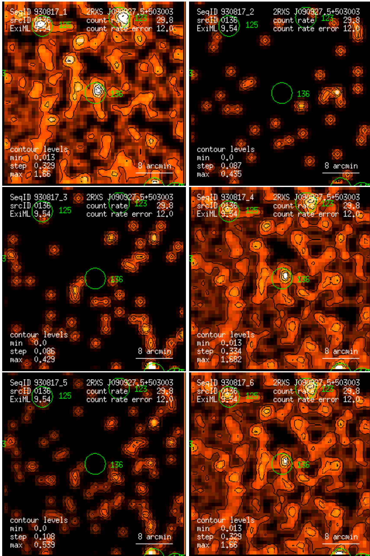
Figure 136: RASS 930817: detection 0136: band rate images, Gaussian filter: (1) PSPC channels 11 – 41, (2) 52 – 90, (3) 91 – 201, (4) 11 – 235, (5) 52 – 201, (6) 11 – 201. Broad band rates in counts/ks. Band rate contour levels in counts/ks/arcmin 2 .
