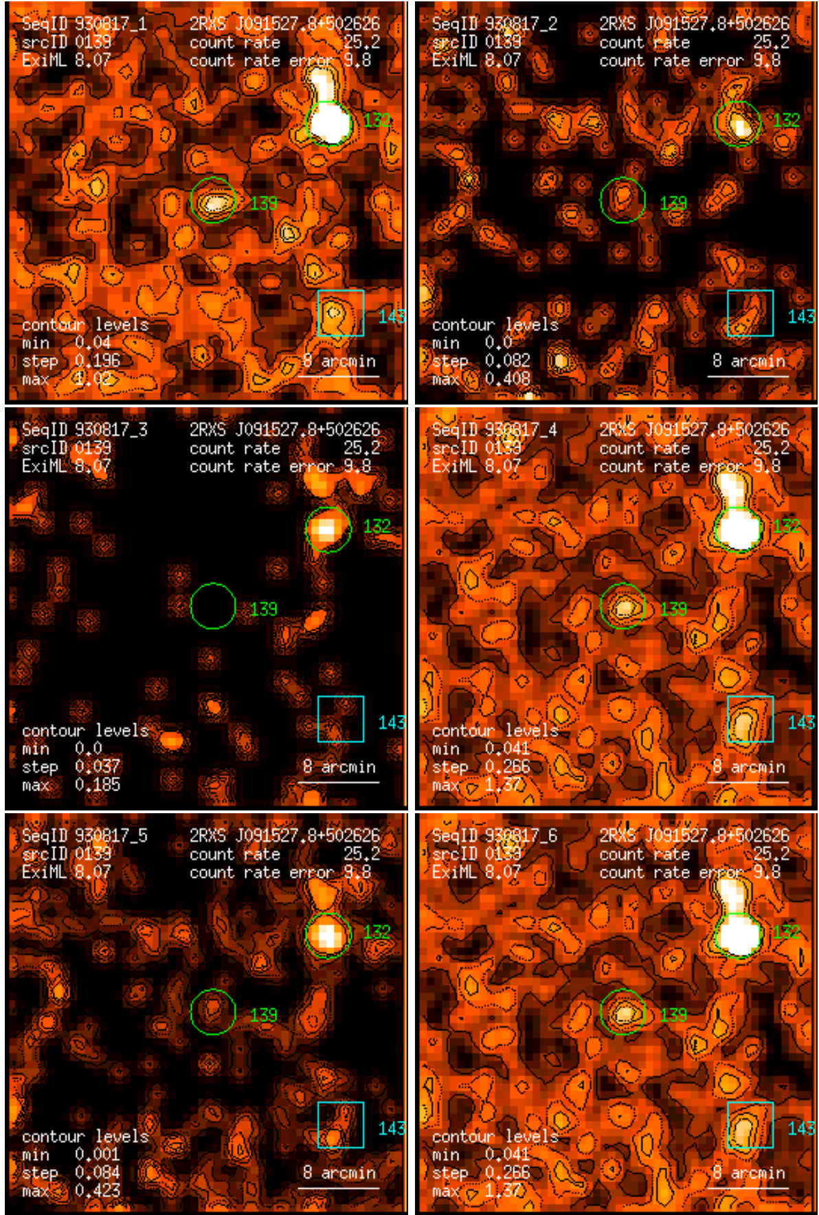
Figure 139: RASS 930817: detection 0139: band rate images, Gaussian filter: (1) PSPC channels 11 – 41, (2) 52 – 90, (3) 91 – 201, (4) 11 – 235, (5) 52 – 201, (6) 11 – 201. Broad band rates in counts/ks. Band rate contour levels in counts/ks/arcmin 2 .
