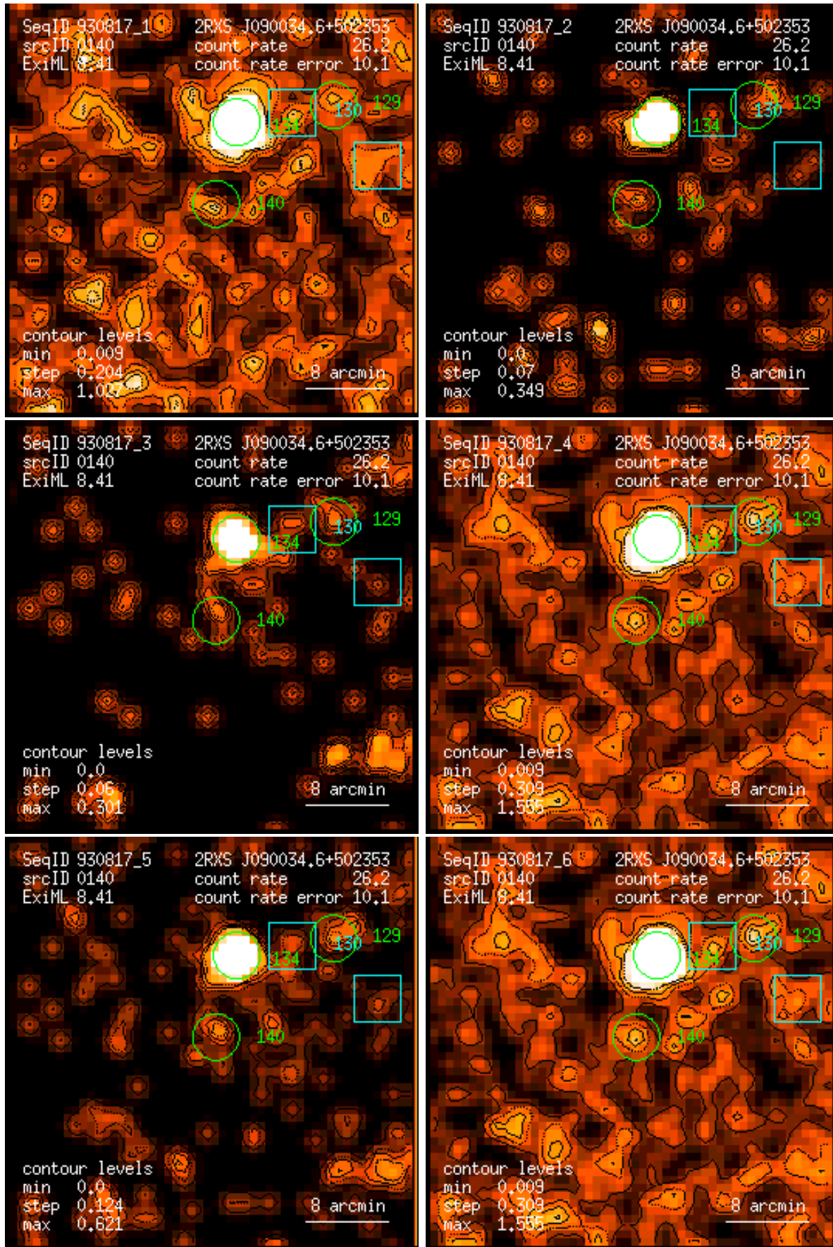
Figure 140: RASS 930817: detection 0140: band rate images, Gaussian filter: (1) PSPC channels 11 – 41, (2) 52 – 90, (3) 91 – 201, (4) 11 – 235, (5) 52 – 201, (6) 11 – 201. Broad band rates in counts/ks. Band rate contour levels in counts/ks/arcmin 2 .
