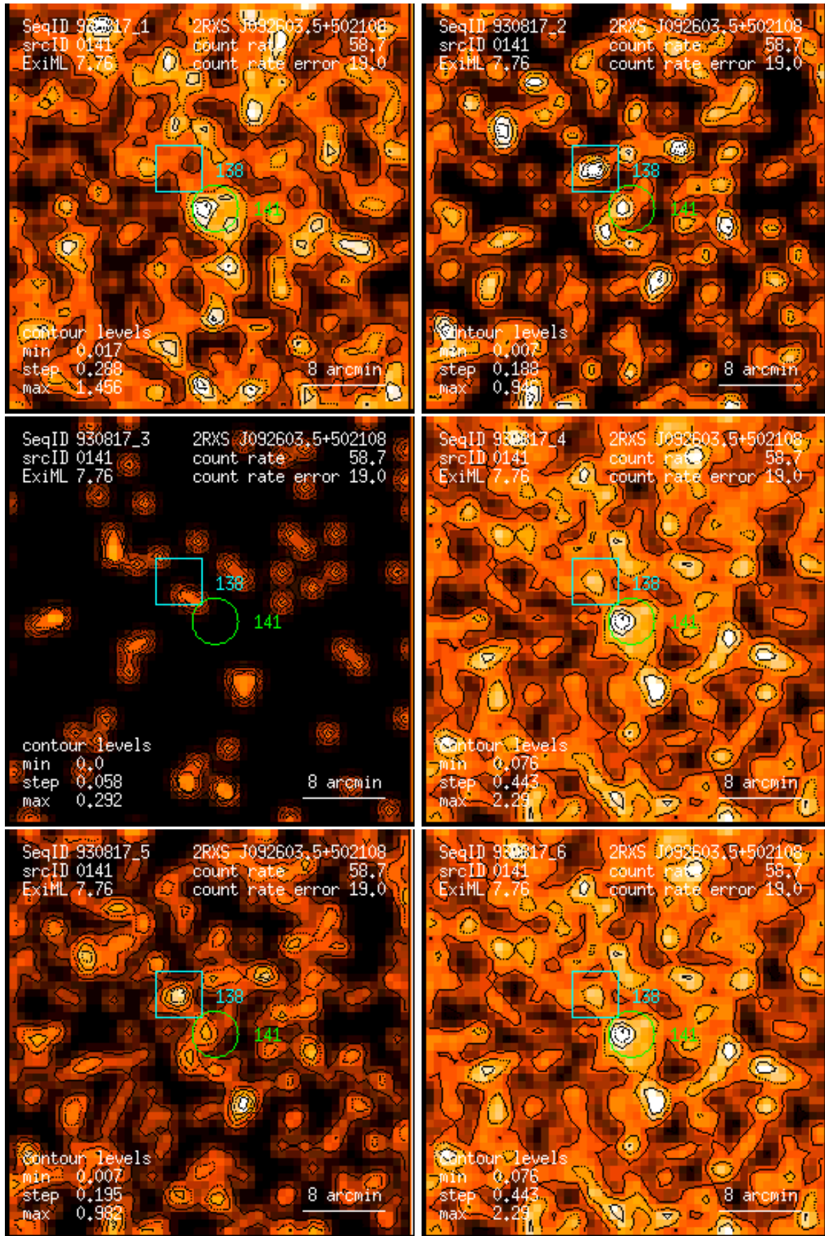
Figure 141: RASS 930817: detection 0141: band rate images, Gaussian filter: (1) PSPC channels 11 – 41, (2) 52 – 90, (3) 91 – 201, (4) 11 – 235, (5) 52 – 201, (6) 11 – 201. Broad band rates in counts/ks. Band rate contour levels in counts/ks/arcmin 2 .
