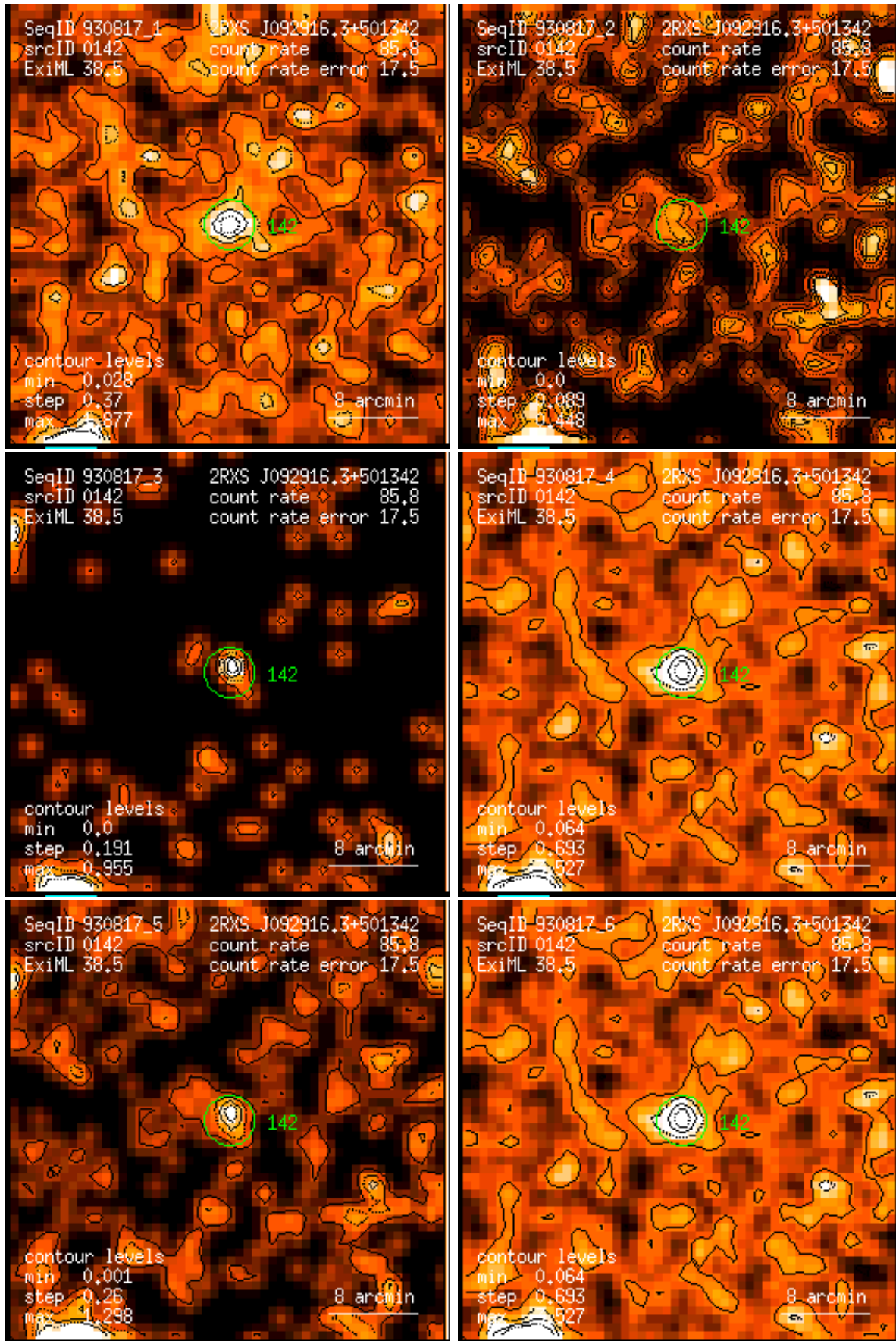
Figure 142: RASS 930817: detection 0142: band rate images, Gaussian filter: (1) PSPC channels 11 – 41, (2) 52 – 90, (3) 91 – 201, (4) 11 – 235, (5) 52 – 201, (6) 11 – 201. Broad band rates in counts/ks. Band rate contour levels in counts/ks/arcmin 2 .
