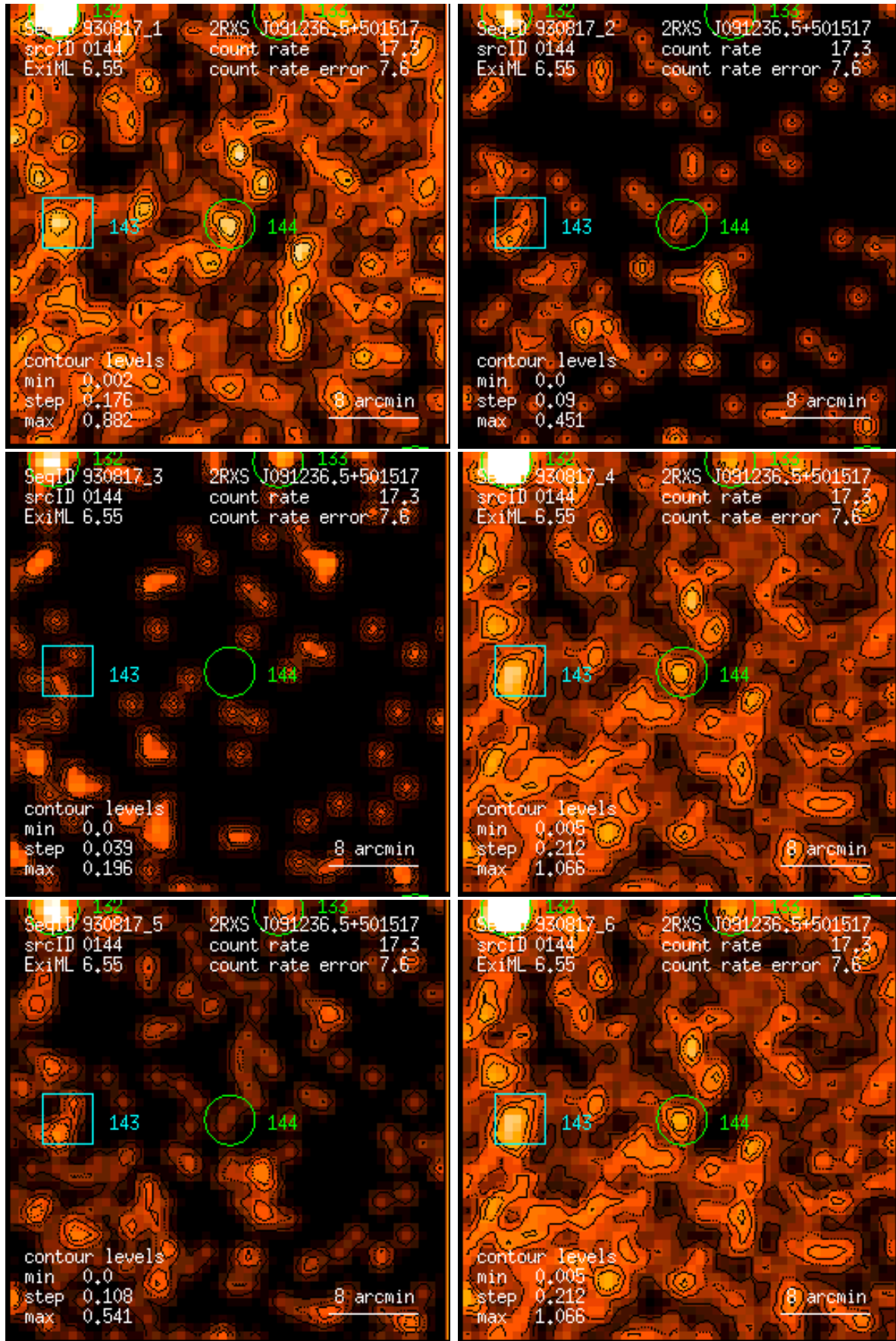
Figure 144: RASS 930817: detection 0144: band rate images, Gaussian filter: (1) PSPC channels 11 – 41, (2) 52 – 90, (3) 91 – 201, (4) 11 – 235, (5) 52 – 201, (6) 11 – 201. Broad band rates in counts/ks. Band rate contour levels in counts/ks/arcmin 2 .
