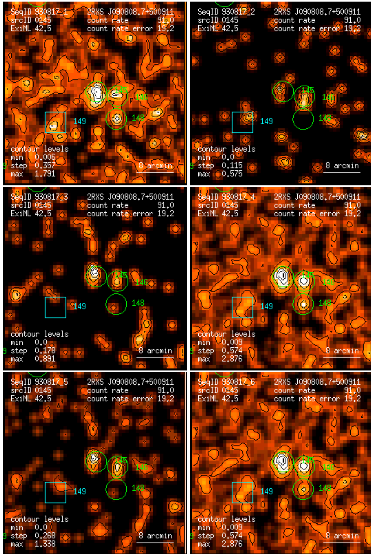
Figure 145: RASS 930817: detection 0145: band rate images, Gaussian filter: (1) PSPC channels 11 – 41, (2) 52 – 90, (3) 91 – 201, (4) 11 – 235, (5) 52 – 201, (6) 11 – 201. Broad band rates in counts/ks. Band rate contour levels in counts/ks/arcmin 2 .
