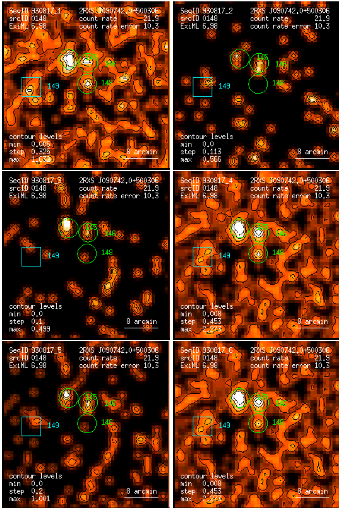
Figure 148: RASS 930817: detection 0148: band rate images, Gaussian filter: (1) PSPC channels 11 – 41, (2) 52 – 90, (3) 91 – 201, (4) 11 – 235, (5) 52 – 201, (6) 11 – 201. Broad band rates in counts/ks. Band rate contour levels in counts/ks/arcmin 2 .
