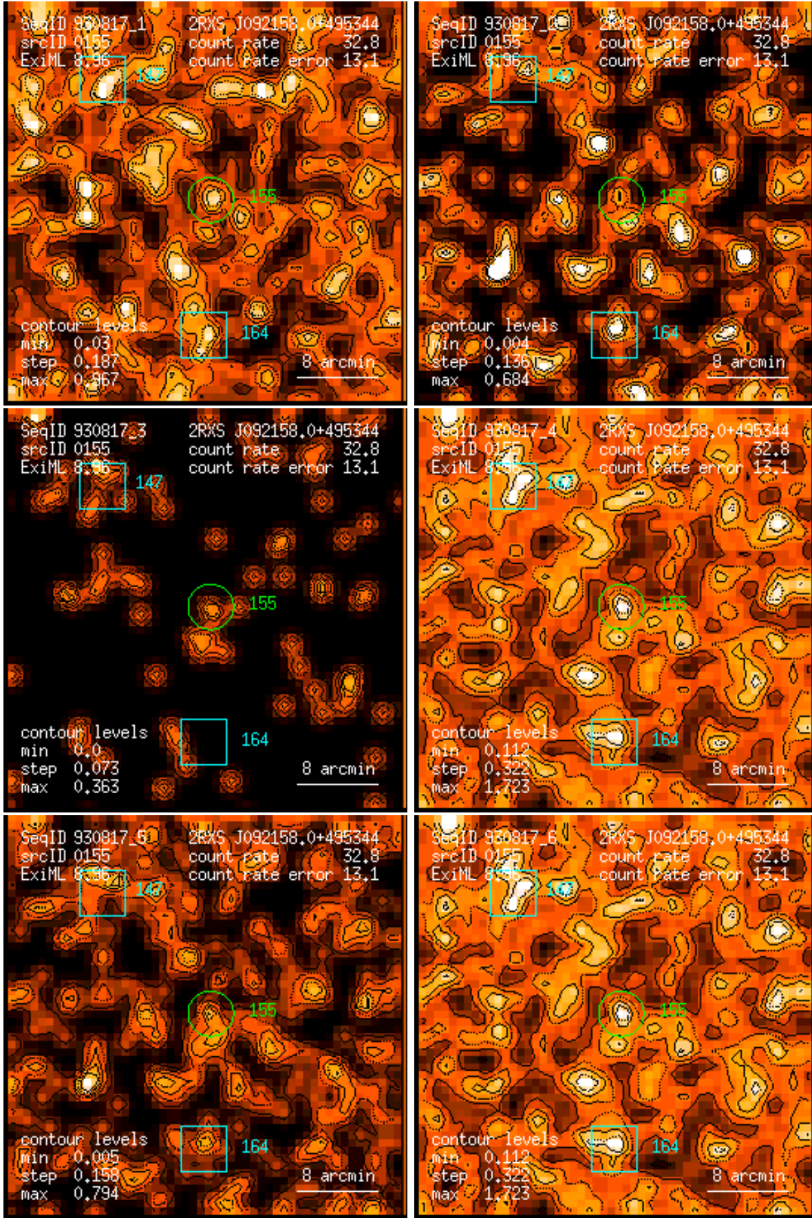
Figure 155: RASS 930817: detection 0155: band rate images, Gaussian filter: (1) PSPC channels 11 – 41, (2) 52 – 90, (3) 91 – 201, (4) 11 – 235, (5) 52 – 201, (6) 11 – 201. Broad band rates in counts/ks. Band rate contour levels in counts/ks/arcmin 2 .
