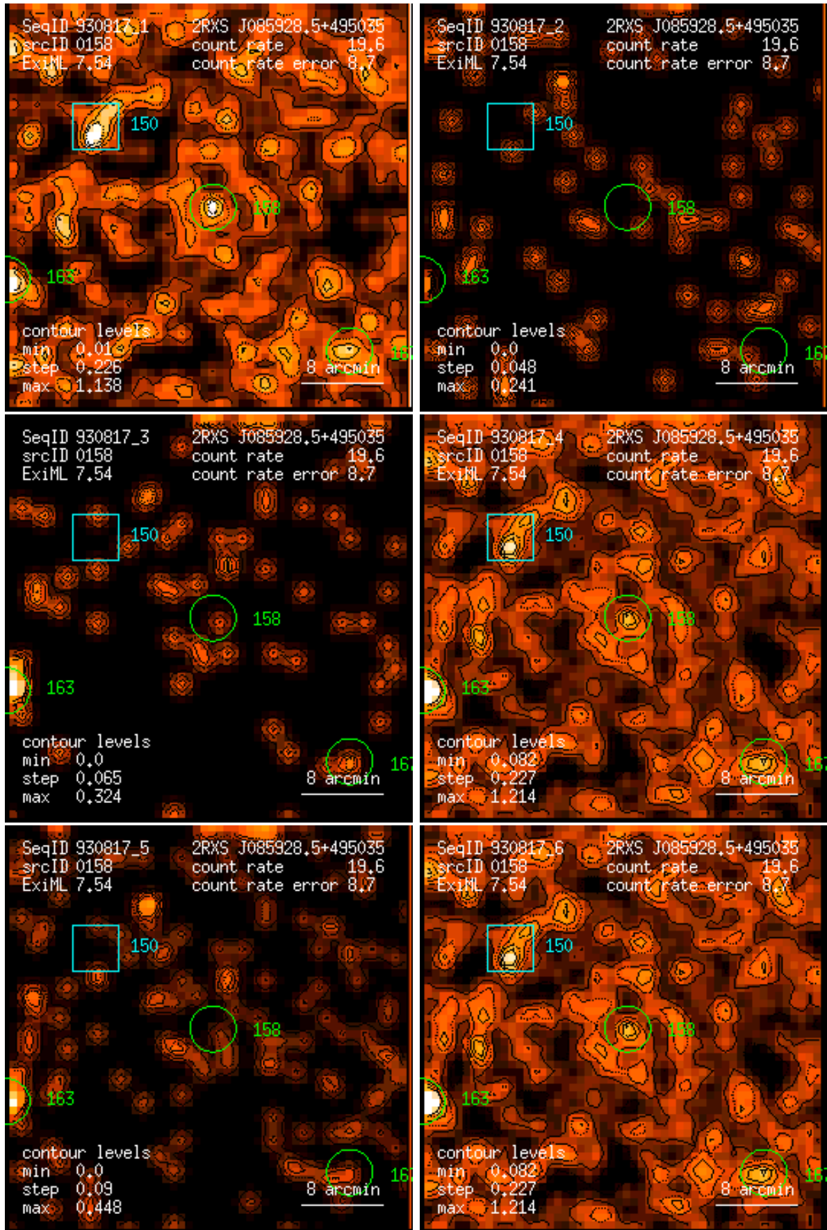
Figure 158: RASS 930817: detection 0158: band rate images, Gaussian filter: (1) PSPC channels 11 – 41, (2) 52 – 90, (3) 91 – 201, (4) 11 – 235, (5) 52 – 201, (6) 11 – 201. Broad band rates in counts/ks. Band rate contour levels in counts/ks/arcmin 2 .
