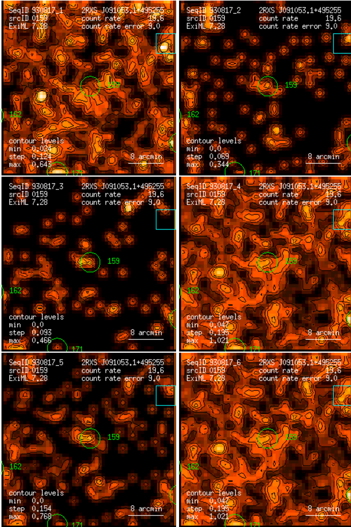
Figure 159: RASS 930817: detection 0159: band rate images, Gaussian filter: (1) PSPC channels 11 – 41, (2) 52 – 90, (3) 91 – 201, (4) 11 – 235, (5) 52 – 201, (6) 11 – 201. Broad band rates in counts/ks. Band rate contour levels in counts/ks/arcmin 2 .
