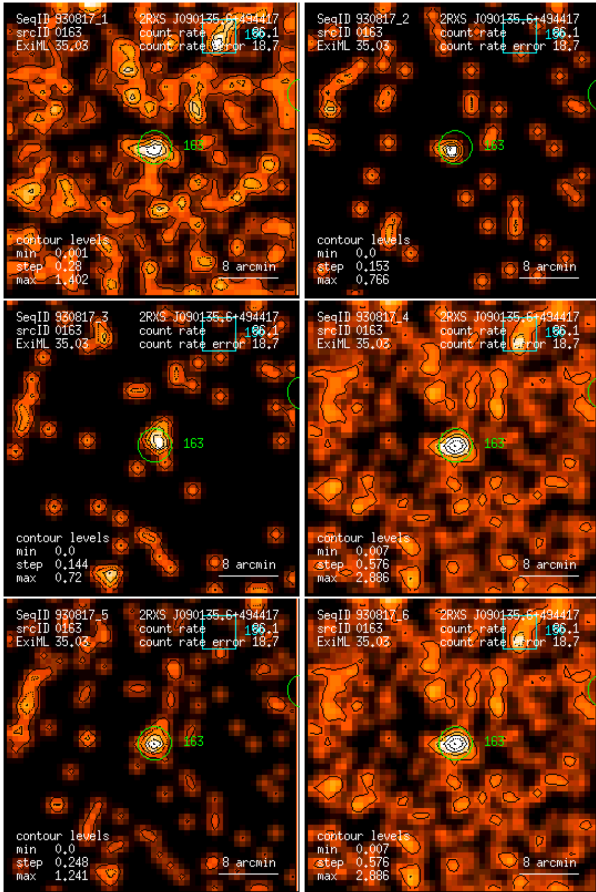
Figure 163: RASS 930817: detection 0163: band rate images, Gaussian filter: (1) PSPC channels 11 – 41, (2) 52 – 90, (3) 91 – 201, (4) 11 – 235, (5) 52 – 201, (6) 11 – 201. Broad band rates in counts/ks. Band rate contour levels in counts/ks/arcmin 2 .
