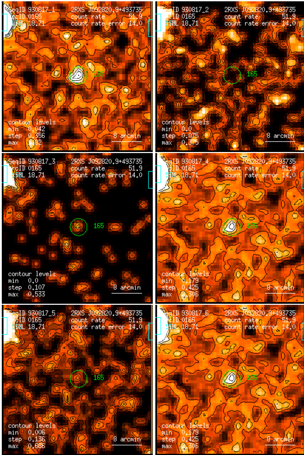
Figure 165: RASS 930817: detection 0165: band rate images, Gaussian filter: (1) PSPC channels 11 – 41, (2) 52 – 90, (3) 91 – 201, (4) 11 – 235, (5) 52 – 201, (6) 11 – 201. Broad band rates in counts/ks. Band rate contour levels in counts/ks/arcmin 2 .
