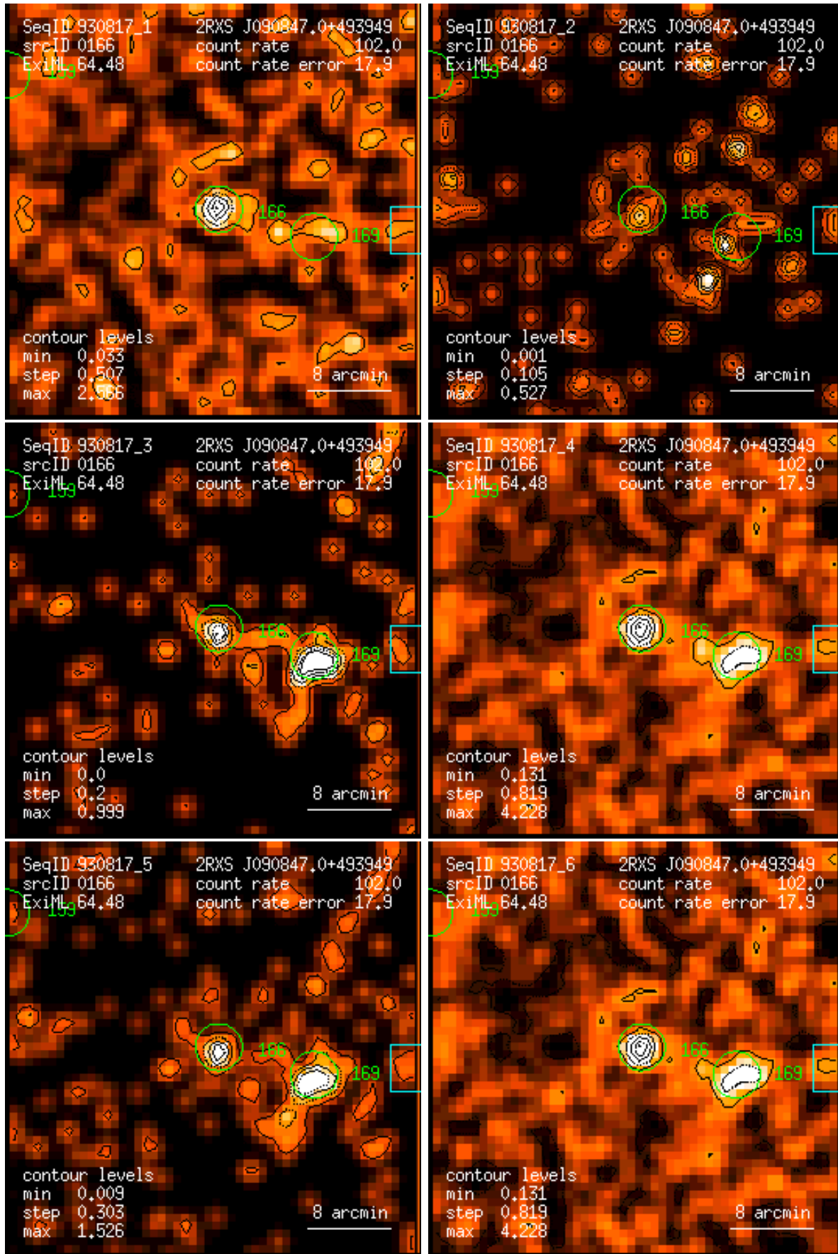
Figure 166: RASS 930817: detection 0166: band rate images, Gaussian filter: (1) PSPC channels 11 – 41, (2) 52 – 90, (3) 91 – 201, (4) 11 – 235, (5) 52 – 201, (6) 11 – 201. Broad band rates in counts/ks. Band rate contour levels in counts/ks/arcmin 2 .
