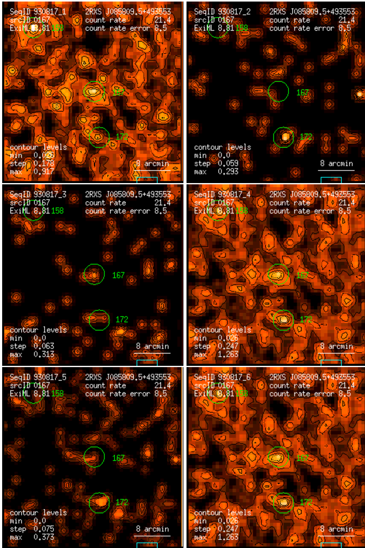
Figure 167: RASS 930817: detection 0167: band rate images, Gaussian filter: (1) PSPC channels 11 – 41, (2) 52 – 90, (3) 91 – 201, (4) 11 – 235, (5) 52 – 201, (6) 11 – 201. Broad band rates in counts/ks. Band rate contour levels in counts/ks/arcmin 2 .
