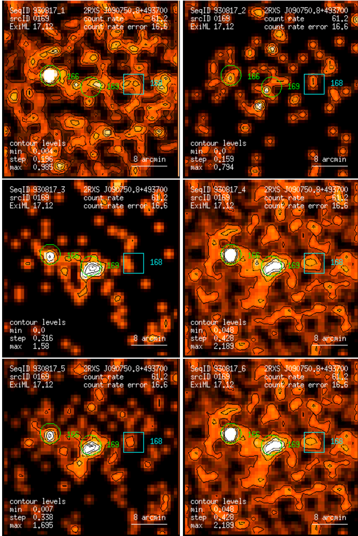
Figure 169: RASS 930817: detection 0169: band rate images, Gaussian filter: (1) PSPC channels 11 – 41, (2) 52 – 90, (3) 91 – 201, (4) 11 – 235, (5) 52 – 201, (6) 11 – 201. Broad band rates in counts/ks. Band rate contour levels in counts/ks/arcmin 2 .
