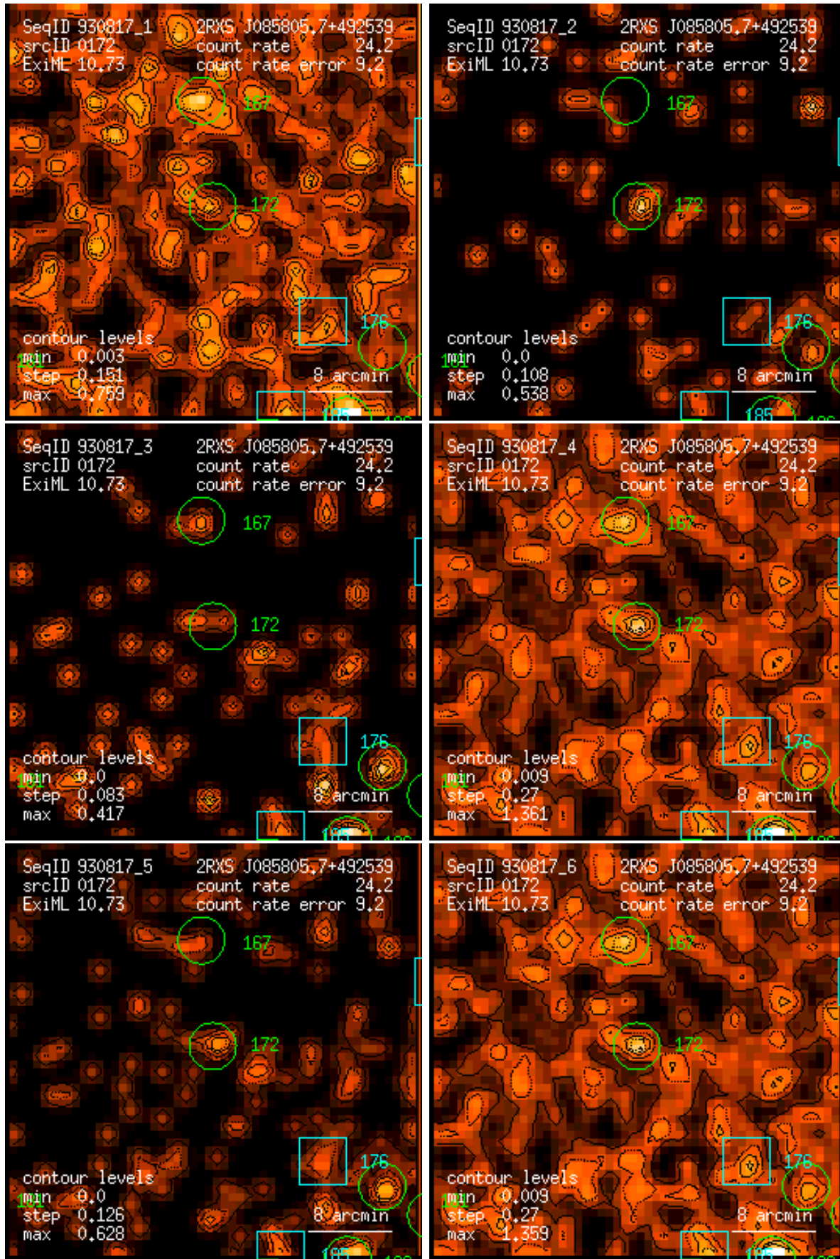
Figure 172: RASS 930817: detection 0172: band rate images, Gaussian filter: (1) PSPC channels 11 – 41, (2) 52 – 90, (3) 91 – 201, (4) 11 – 235, (5) 52 – 201, (6) 11 – 201. Broad band rates in counts/ks. Band rate contour levels in counts/ks/arcmin 2 .
