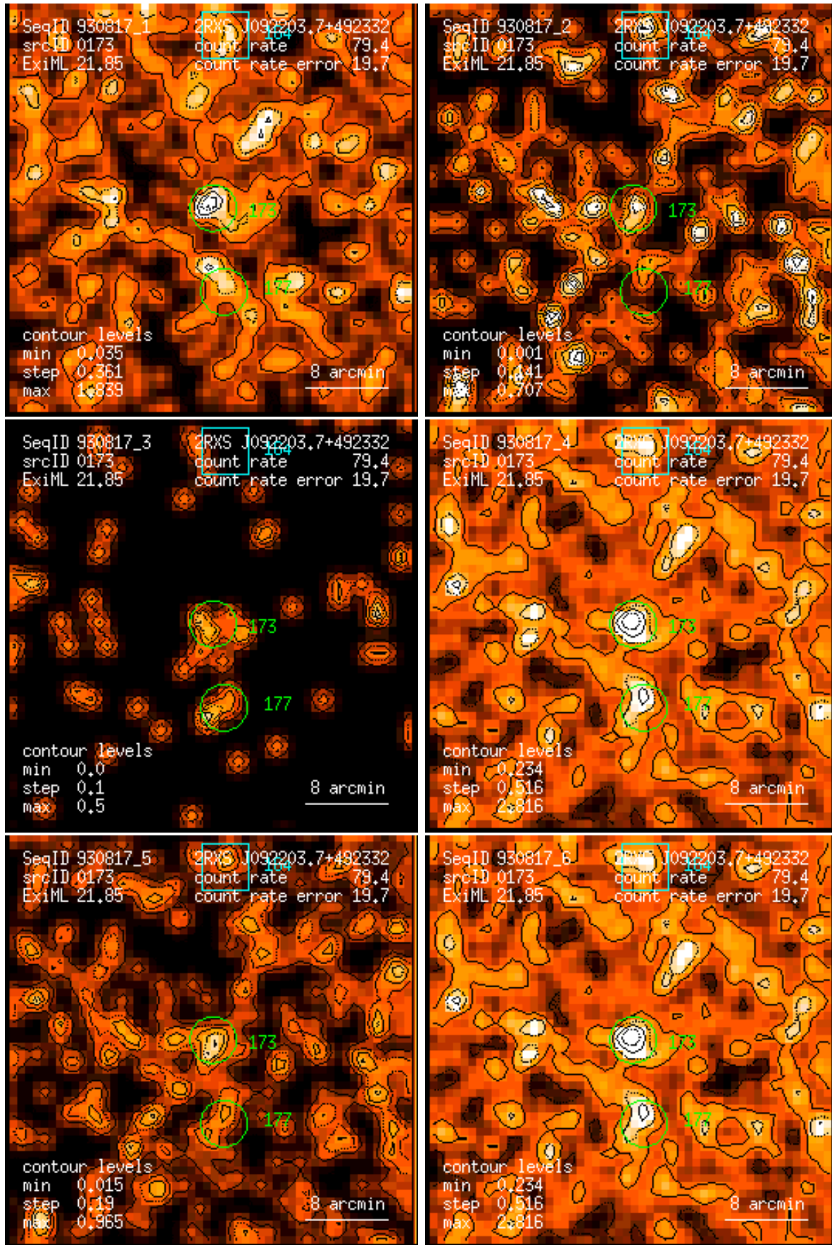
Figure 173: RASS 930817: detection 0173: band rate images, Gaussian filter: (1) PSPC channels 11 – 41, (2) 52 – 90, (3) 91 – 201, (4) 11 – 235, (5) 52 – 201, (6) 11 – 201. Broad band rates in counts/ks. Band rate contour levels in counts/ks/arcmin 2 .
