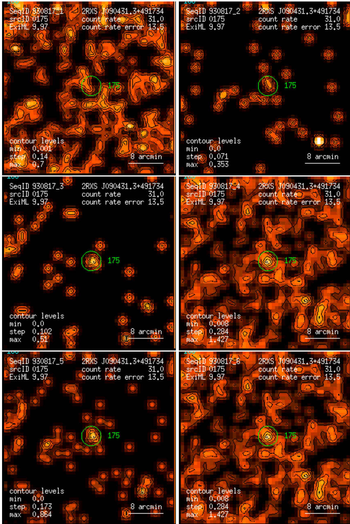
Figure 175: RASS 930817: detection 0175: band rate images, Gaussian filter: (1) PSPC channels 11 – 41, (2) 52 – 90, (3) 91 – 201, (4) 11 – 235, (5) 52 – 201, (6) 11 – 201. Broad band rates in counts/ks. Band rate contour levels in counts/ks/arcmin 2 .
