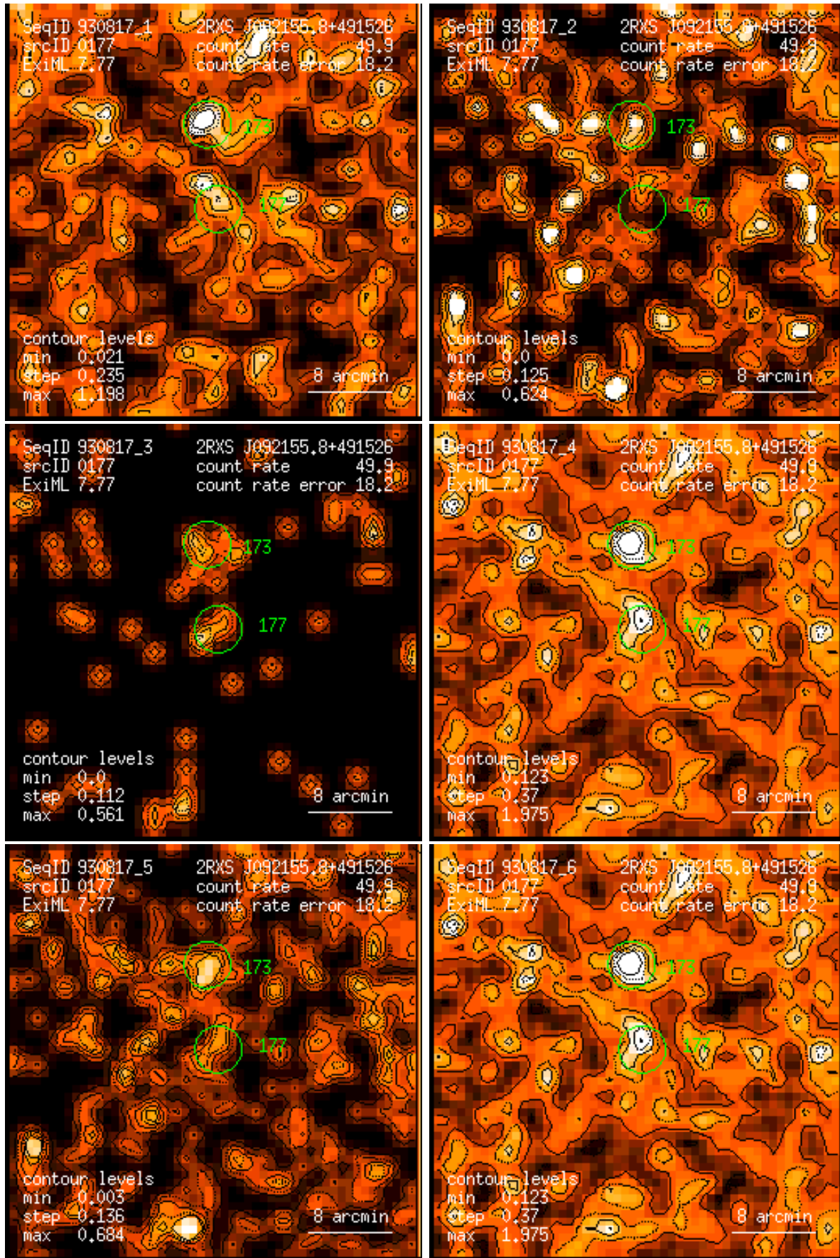
Figure 177: RASS 930817: detection 0177: band rate images, Gaussian filter: (1) PSPC channels 11 – 41, (2) 52 – 90, (3) 91 – 201, (4) 11 – 235, (5) 52 – 201, (6) 11 – 201. Broad band rates in counts/ks. Band rate contour levels in counts/ks/arcmin 2 .
