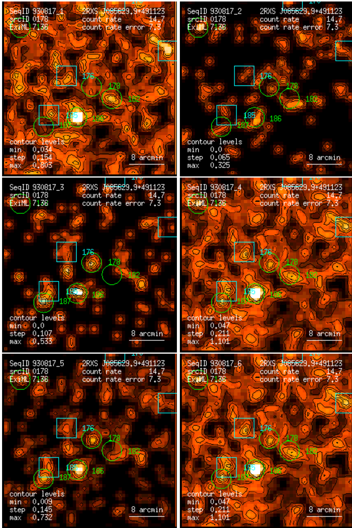
Figure 178: RASS 930817: detection 0178: band rate images, Gaussian filter: (1) PSPC channels 11 – 41, (2) 52 – 90, (3) 91 – 201, (4) 11 – 235, (5) 52 – 201, (6) 11 – 201. Broad band rates in counts/ks. Band rate contour levels in counts/ks/arcmin 2 .
