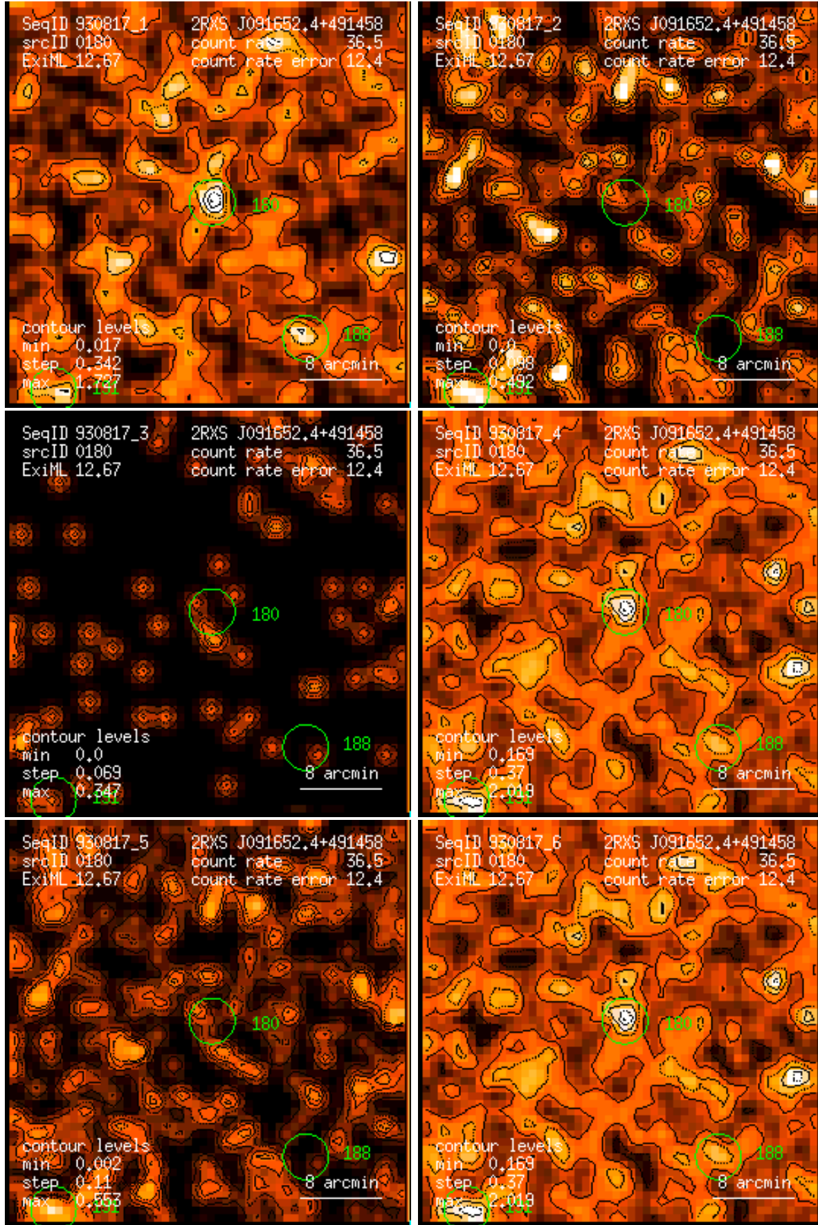
Figure 180: RASS 930817: detection 0180: band rate images, Gaussian filter: (1) PSPC channels 11 – 41, (2) 52 – 90, (3) 91 – 201, (4) 11 – 235, (5) 52 – 201, (6) 11 – 201. Broad band rates in counts/ks. Band rate contour levels in counts/ks/arcmin 2 .
