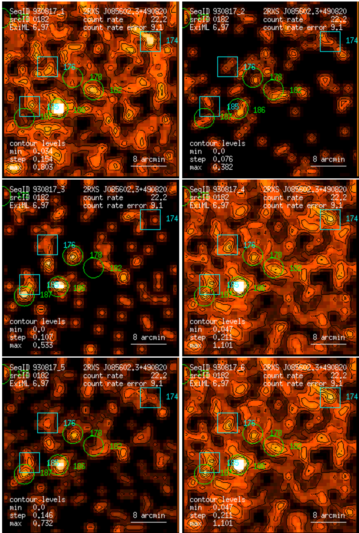
Figure 182: RASS 930817: detection 0182: band rate images, Gaussian filter: (1) PSPC channels 11 – 41, (2) 52 – 90, (3) 91 – 201, (4) 11 – 235, (5) 52 – 201, (6) 11 – 201. Broad band rates in counts/ks. Band rate contour levels in counts/ks/arcmin 2 .
