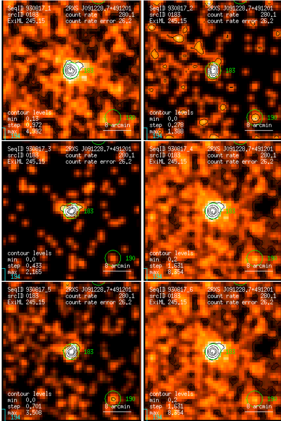
Figure 183: RASS 930817: detection 0183: band rate images, Gaussian filter: (1) PSPC channels 11 – 41, (2) 52 – 90, (3) 91 – 201, (4) 11 – 235, (5) 52 – 201, (6) 11 – 201. Broad band rates in counts/ks. Band rate contour levels in counts/ks/arcmin 2 .
