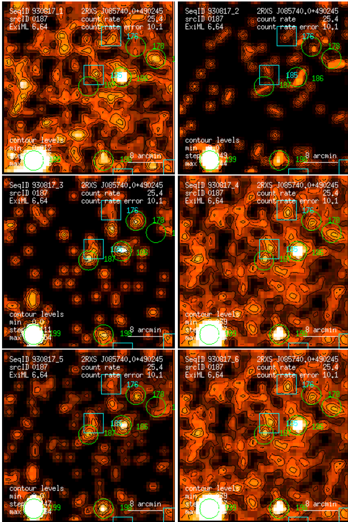
Figure 187: RASS 930817: detection 0187: band rate images, Gaussian filter: (1) PSPC channels 11 – 41, (2) 52 – 90, (3) 91 – 201, (4) 11 – 235, (5) 52 – 201, (6) 11 – 201. Broad band rates in counts/ks. Band rate contour levels in counts/ks/arcmin 2 .
