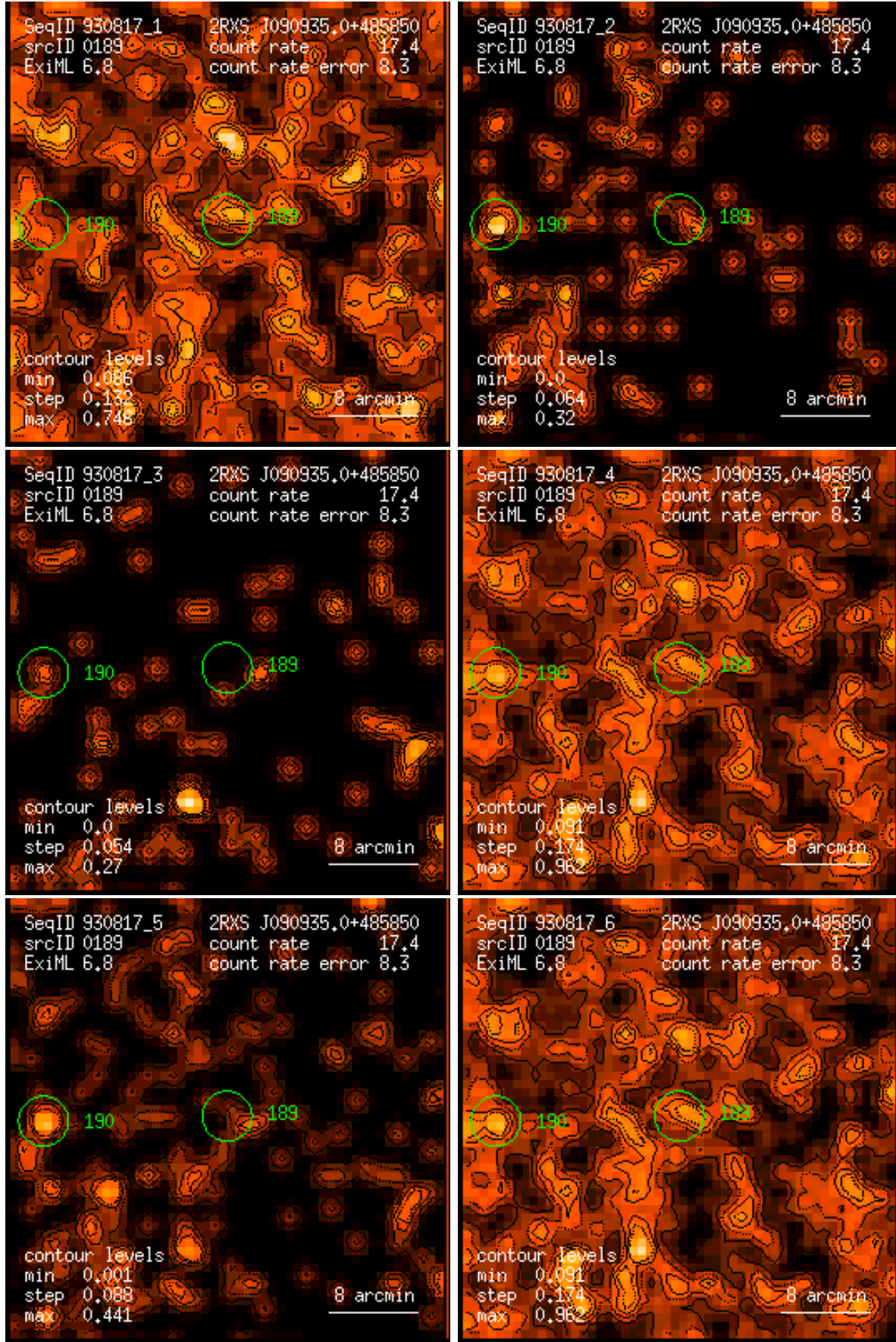
Figure 189: RASS 930817: detection 0189: band rate images, Gaussian filter: (1) PSPC channels 11 – 41, (2) 52 – 90, (3) 91 – 201, (4) 11 – 235, (5) 52 – 201, (6) 11 – 201. Broad band rates in counts/ks. Band rate contour levels in counts/ks/arcmin 2 .
