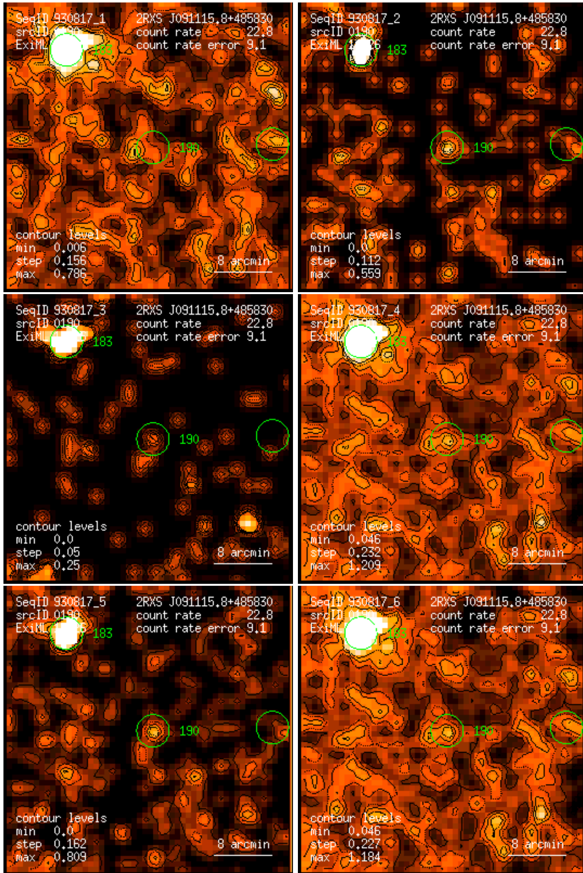
Figure 190: RASS 930817: detection 0190: band rate images, Gaussian filter: (1) PSPC channels 11 – 41, (2) 52 – 90, (3) 91 – 201, (4) 11 – 235, (5) 52 – 201, (6) 11 – 201. Broad band rates in counts/ks. Band rate contour levels in counts/ks/arcmin 2 .
