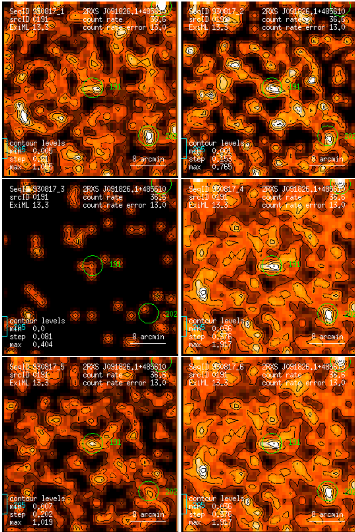
Figure 191: RASS 930817: detection 0191: band rate images, Gaussian filter: (1) PSPC channels 11 – 41, (2) 52 – 90, (3) 91 – 201, (4) 11 – 235, (5) 52 – 201, (6) 11 – 201. Broad band rates in counts/ks. Band rate contour levels in counts/ks/arcmin 2 .
