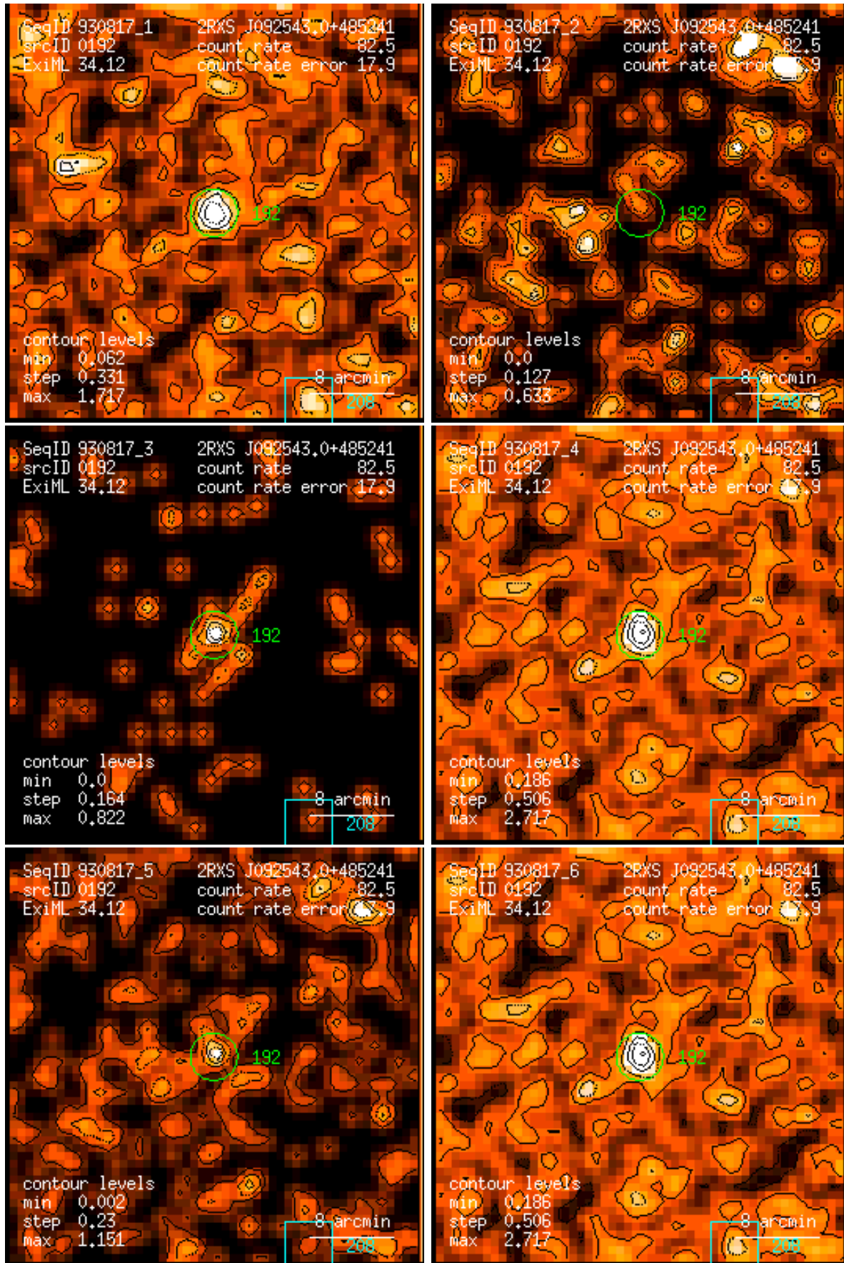
Figure 192: RASS 930817: detection 0192: band rate images, Gaussian filter: (1) PSPC channels 11 – 41, (2) 52 – 90, (3) 91 – 201, (4) 11 – 235, (5) 52 – 201, (6) 11 – 201. Broad band rates in counts/ks. Band rate contour levels in counts/ks/arcmin 2 .
