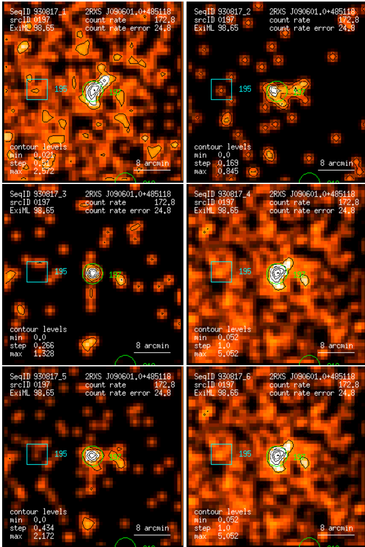
Figure 197: RASS 930817: detection 0197: band rate images, Gaussian filter: (1) PSPC channels 11 – 41, (2) 52 – 90, (3) 91 – 201, (4) 11 – 235, (5) 52 – 201, (6) 11 – 201. Broad band rates in counts/ks. Band rate contour levels in counts/ks/arcmin 2 .
