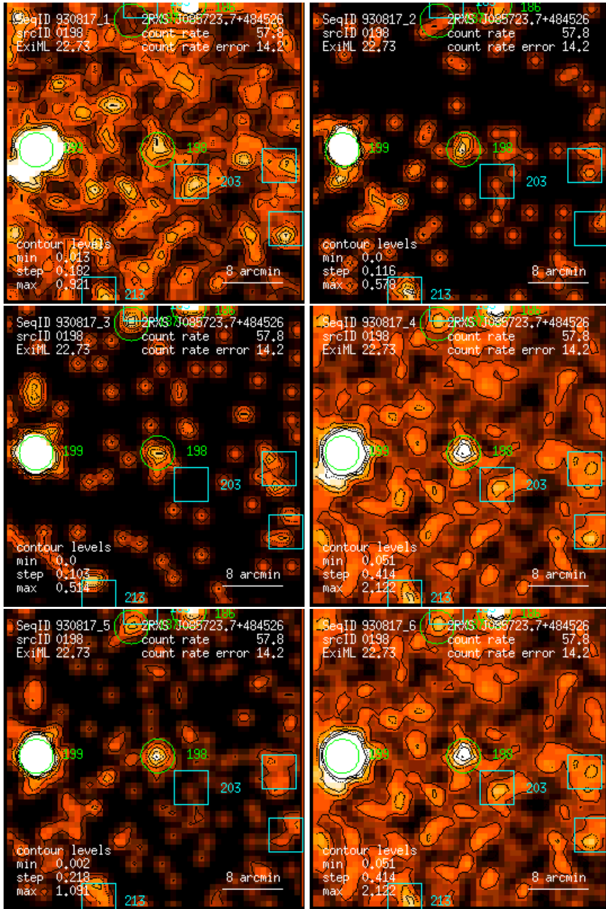
Figure 198: RASS 930817: detection 0198: band rate images, Gaussian filter: (1) PSPC channels 11 – 41, (2) 52 – 90, (3) 91 – 201, (4) 11 – 235, (5) 52 – 201, (6) 11 – 201. Broad band rates in counts/ks. Band rate contour levels in counts/ks/arcmin 2 .
