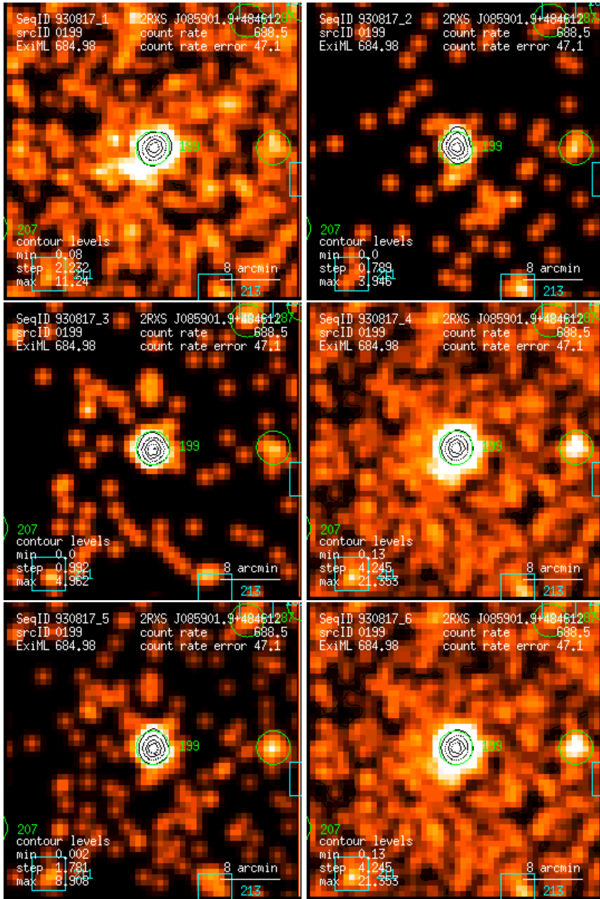
Figure 199: RASS 930817: detection 0199: band rate images, Gaussian filter: (1) PSPC channels 11 – 41, (2) 52 – 90, (3) 91 – 201, (4) 11 – 235, (5) 52 – 201, (6) 11 – 201. Broad band rates in counts/ks. Band rate contour levels in counts/ks/arcmin 2 .
