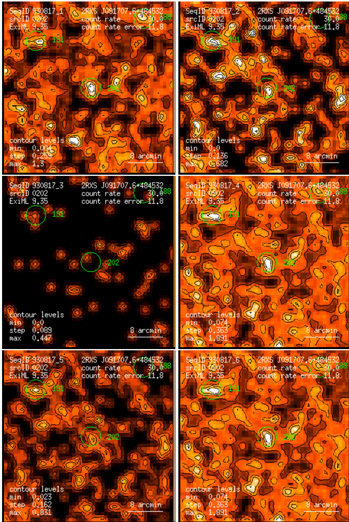
Figure 202: RASS 930817: detection 0202: band rate images, Gaussian filter: (1) PSPC channels 11 – 41, (2) 52 – 90, (3) 91 – 201, (4) 11 – 235, (5) 52 – 201, (6) 11 – 201. Broad band rates in counts/ks. Band rate contour levels in counts/ks/arcmin 2 .
