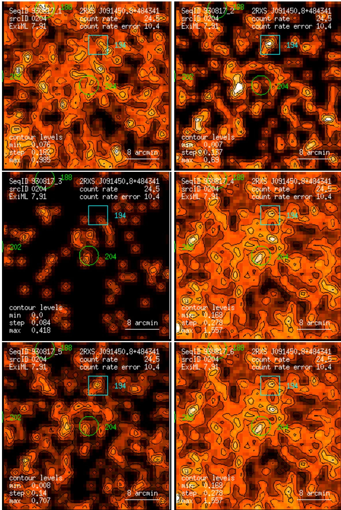
Figure 204: RASS 930817: detection 0204: band rate images, Gaussian filter: (1) PSPC channels 11 – 41, (2) 52 – 90, (3) 91 – 201, (4) 11 – 235, (5) 52 – 201, (6) 11 – 201. Broad band rates in counts/ks. Band rate contour levels in counts/ks/arcmin 2 .
