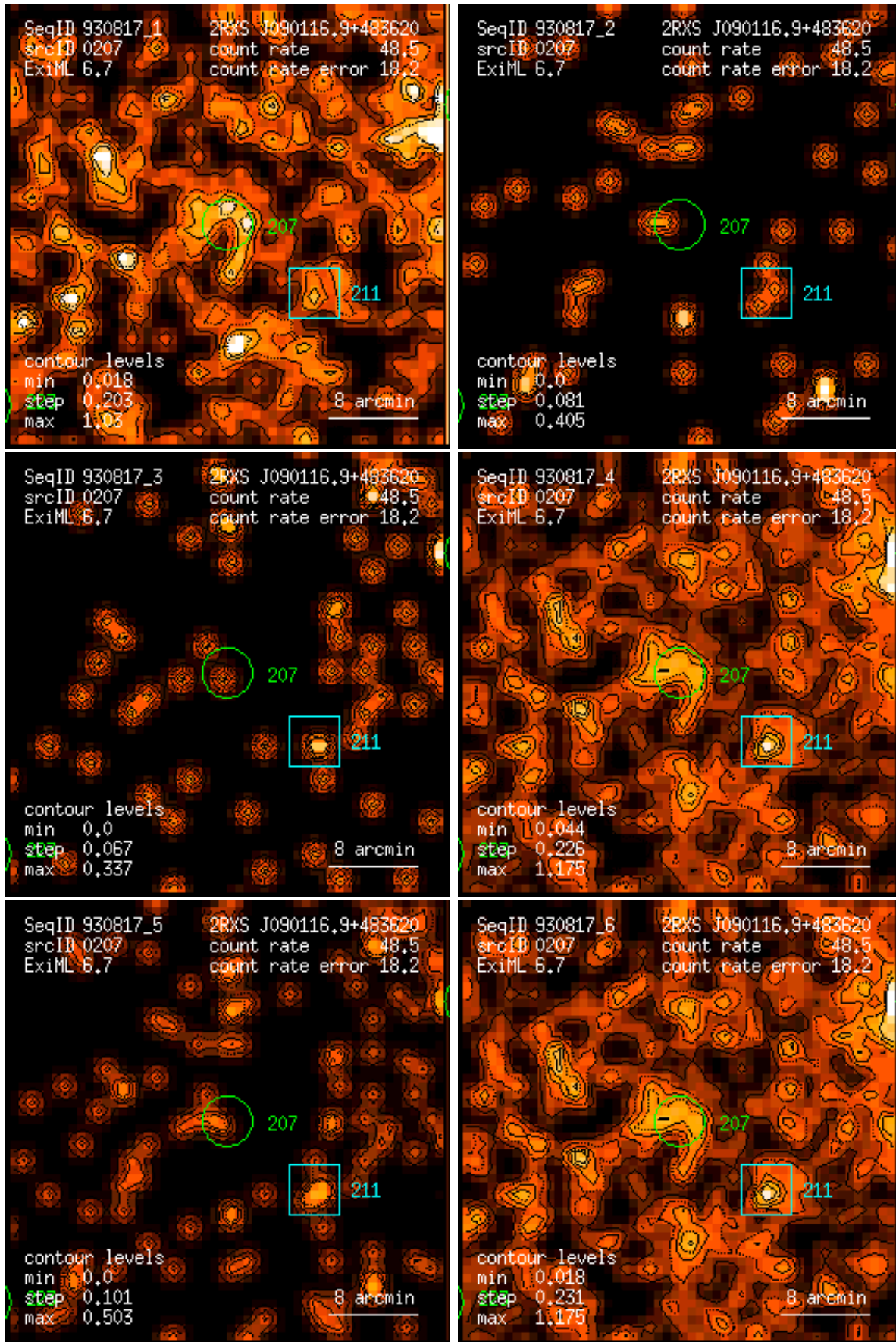
Figure 207: RASS 930817: detection 0207: band rate images, Gaussian filter: (1) PSPC channels 11 – 41, (2) 52 – 90, (3) 91 – 201, (4) 11 – 235, (5) 52 – 201, (6) 11 – 201. Broad band rates in counts/ks. Band rate contour levels in counts/ks/arcmin 2 .
