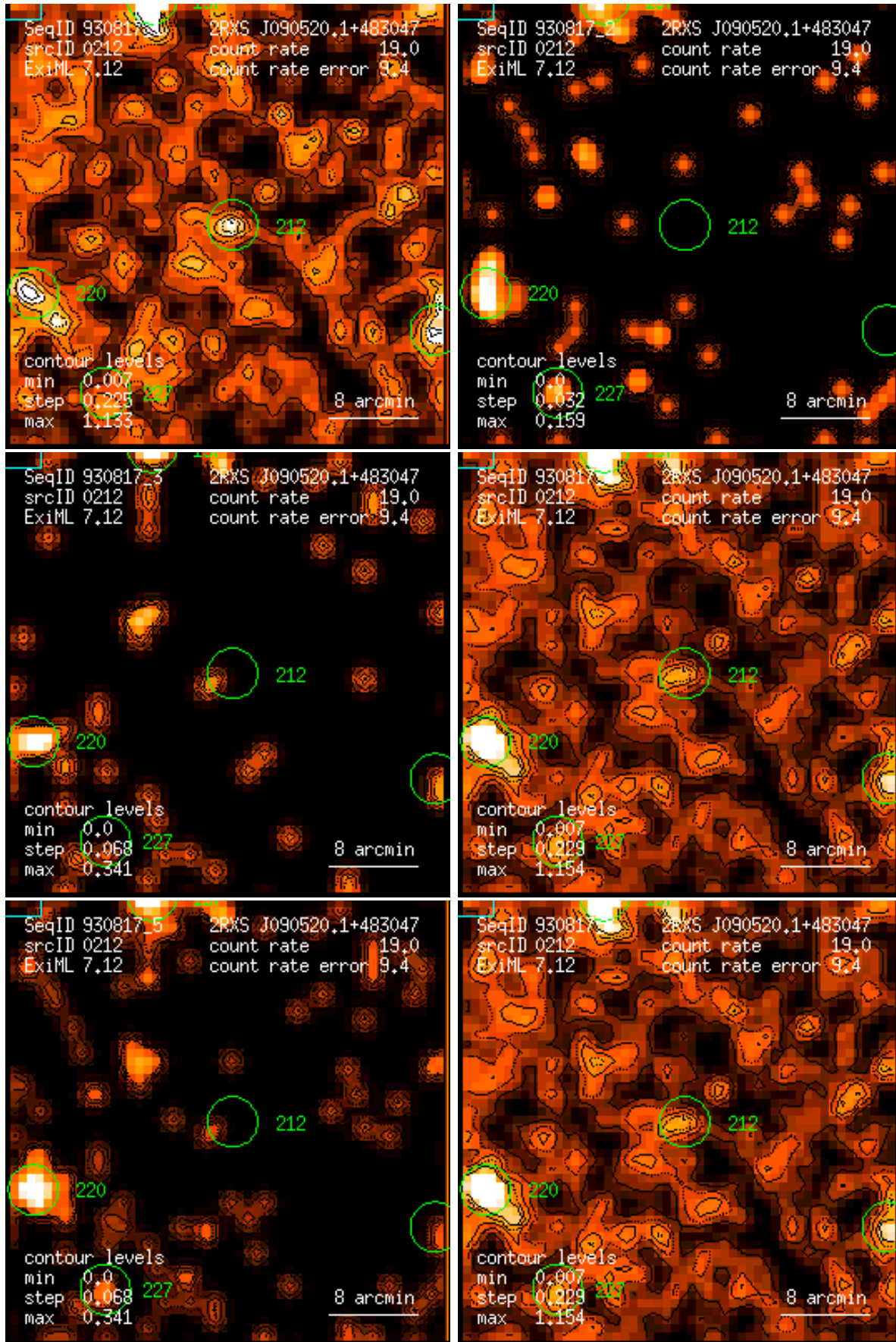
Figure 212: RASS 930817: detection 0212: band rate images, Gaussian filter: (1) PSPC channels 11 – 41, (2) 52 – 90, (3) 91 – 201, (4) 11 – 235, (5) 52 – 201, (6) 11 – 201. Broad band rates in counts/ks. Band rate contour levels in counts/ks/arcmin 2 .
