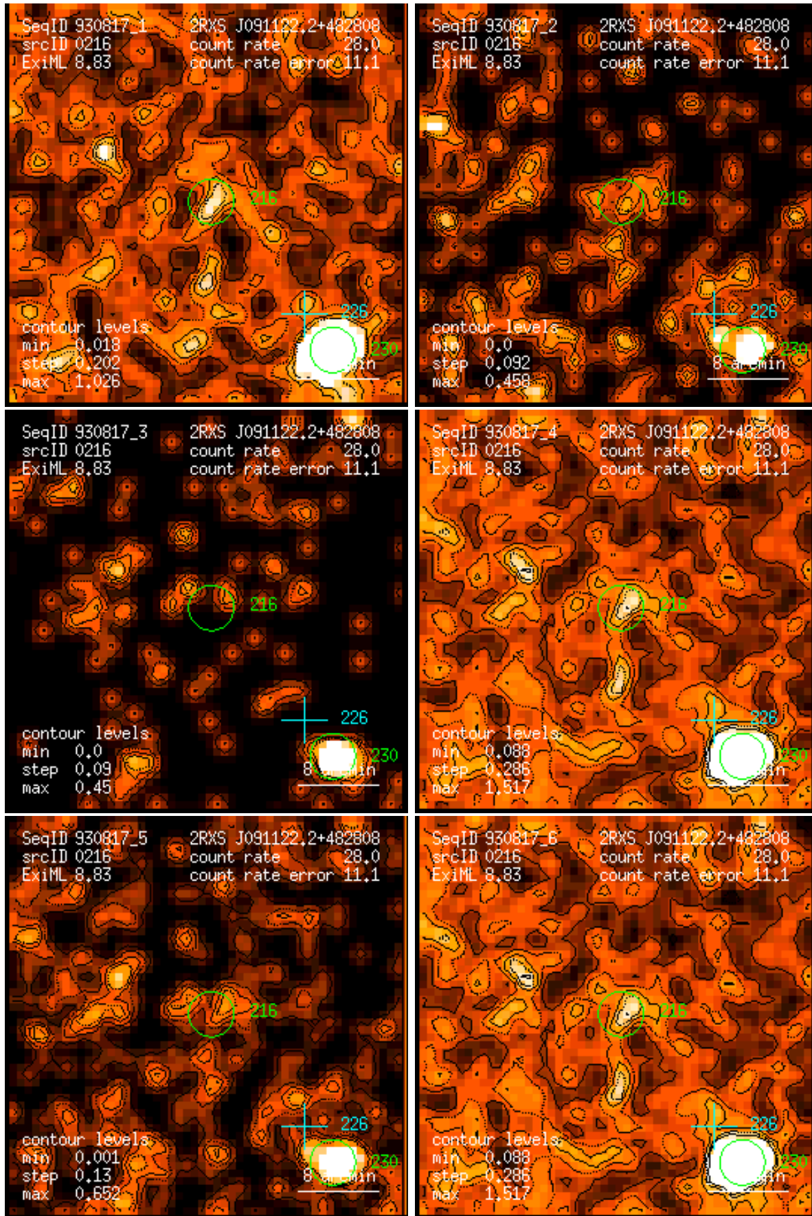
Figure 216: RASS 930817: detection 0216: band rate images, Gaussian filter: (1) PSPC channels 11 – 41, (2) 52 – 90, (3) 91 – 201, (4) 11 – 235, (5) 52 – 201, (6) 11 – 201. Broad band rates in counts/ks. Band rate contour levels in counts/ks/arcmin 2 .
