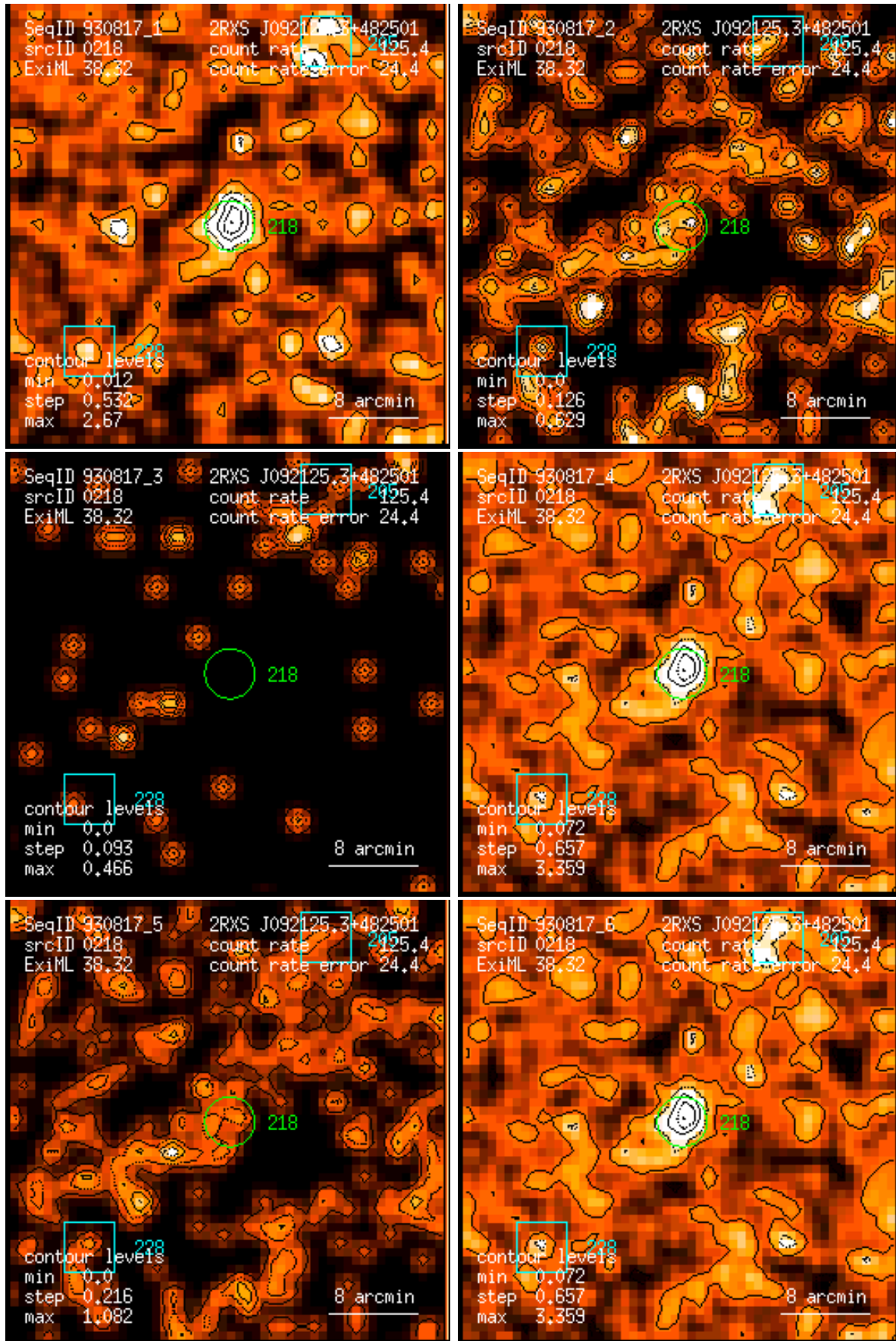
Figure 218: RASS 930817: detection 0218: band rate images, Gaussian filter: (1) PSPC channels 11 – 41, (2) 52 – 90, (3) 91 – 201, (4) 11 – 235, (5) 52 – 201, (6) 11 – 201. Broad band rates in counts/ks. Band rate contour levels in counts/ks/arcmin 2 .
