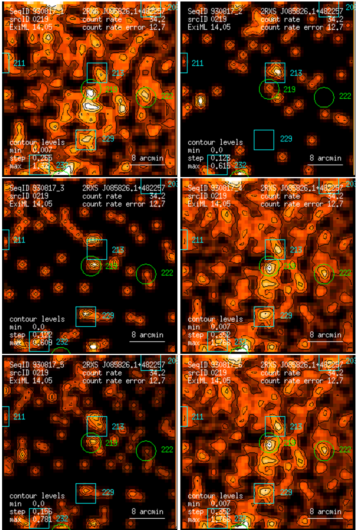
Figure 219: RASS 930817: detection 0219: band rate images, Gaussian filter: (1) PSPC channels 11 – 41, (2) 52 – 90, (3) 91 – 201, (4) 11 – 235, (5) 52 – 201, (6) 11 – 201. Broad band rates in counts/ks. Band rate contour levels in counts/ks/arcmin 2 .
